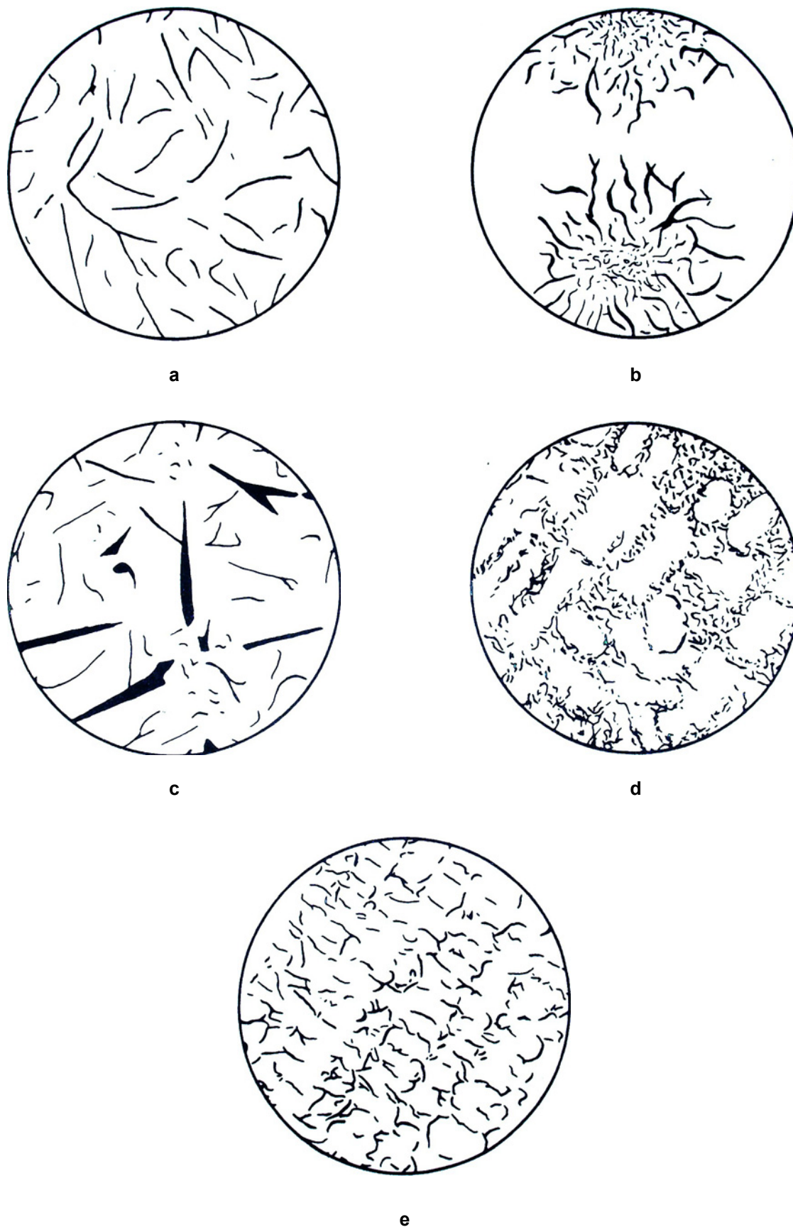
Figure 5 — Reference diagrams for graphite distribution
