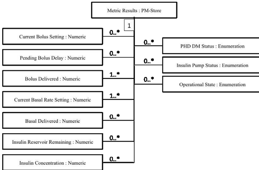
Figure 6—Insulin pump—metric persistent store model
