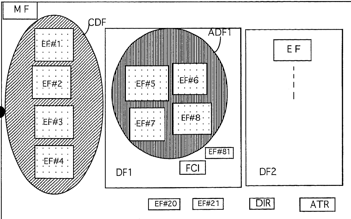
Figure 3 - CDF ISO 9992 + ADF ISO 9992 + DF ISO/IEC 7816-4
