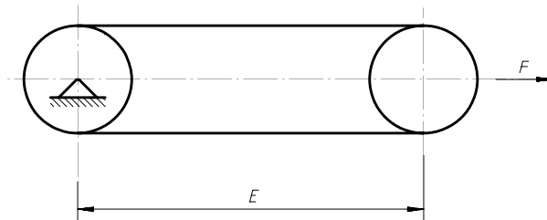
Figure 5 — Measuring fixture to determine effective length
