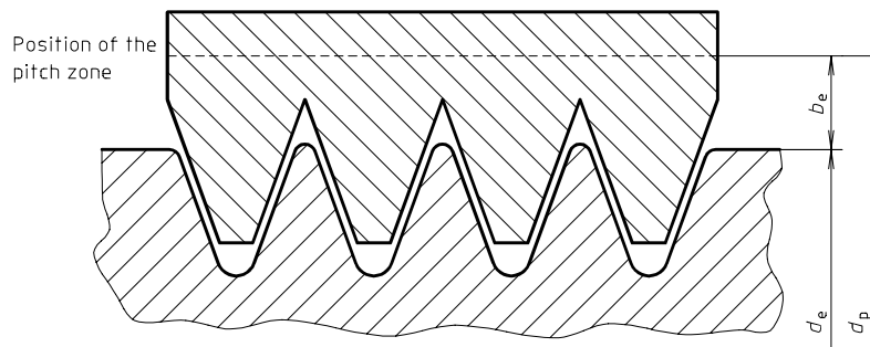
Figure 3 — Determination of pitch diameter
