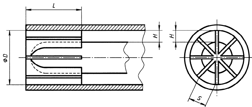
Figure E.5 — Meter dimensions defining similarity for various size meters
