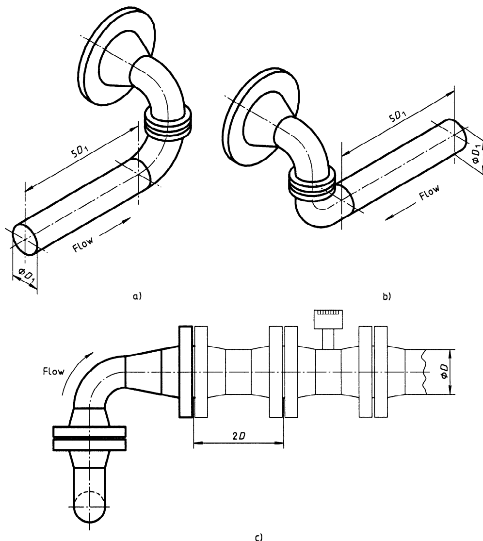
Figure E.1 — Piping configurations for tests at low level perturbation
