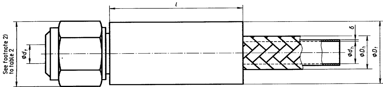
Figure 1 — Hose and fitting dimensions
