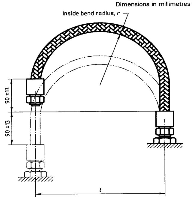
Figure 2 — Test setup for flexure test
