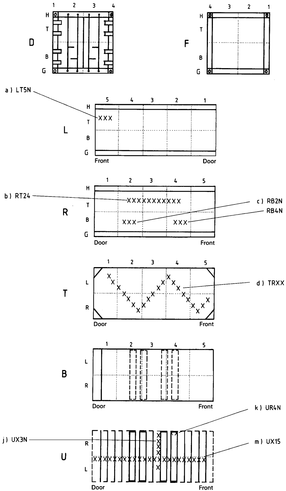
Figure C.1 — Examples of location coding for containers
