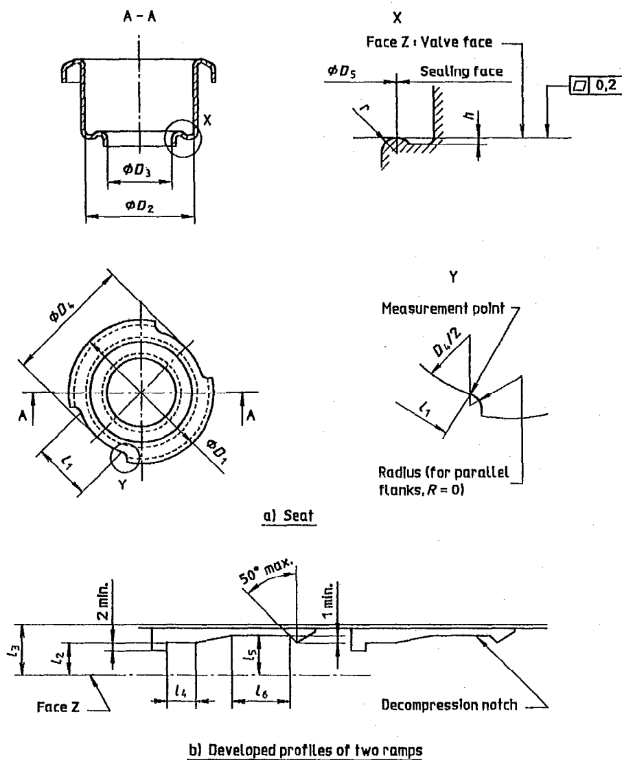
Figure A.1 — Seat with clamping ramps
