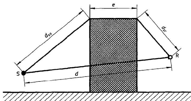
Figure 6 — Geometrical quantities for determining the pathlength difference for single diffraction
