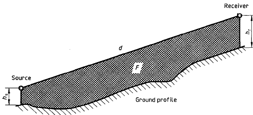
Figure 3 — Method for evaluating the mean height h_m
