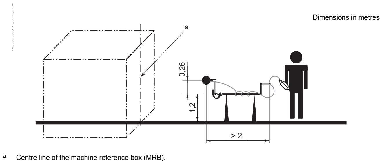
Figure B.1 — Electrical conduit apparatus for measurement
