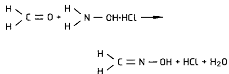
Oximation reaction
