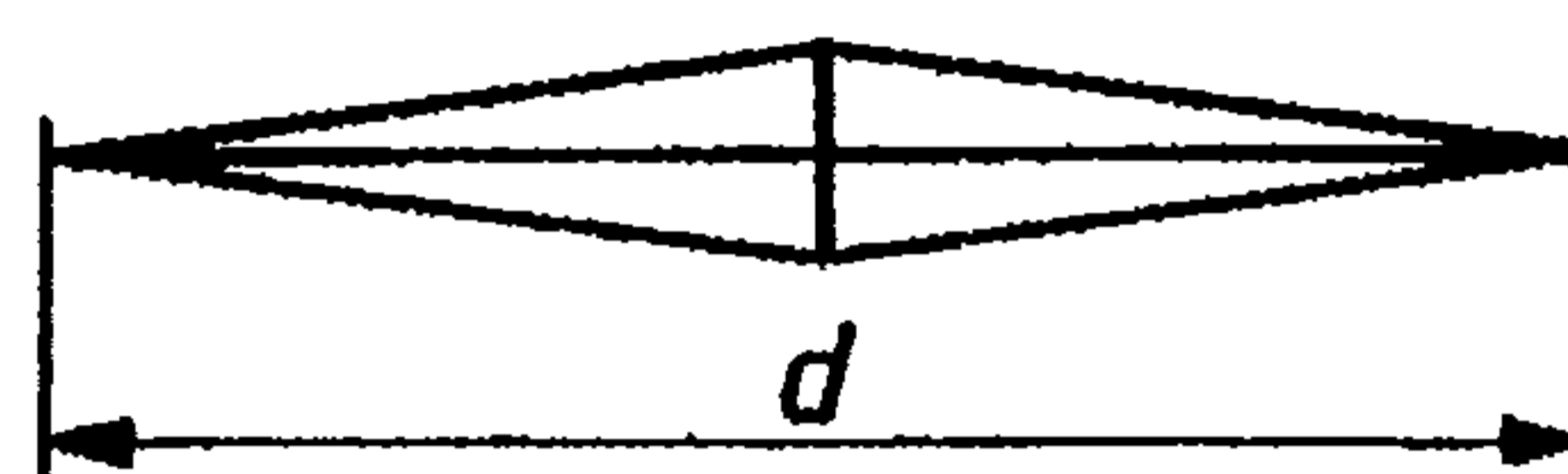
Figure 1 — Base area of the indentation produced by the Knoop indenter
