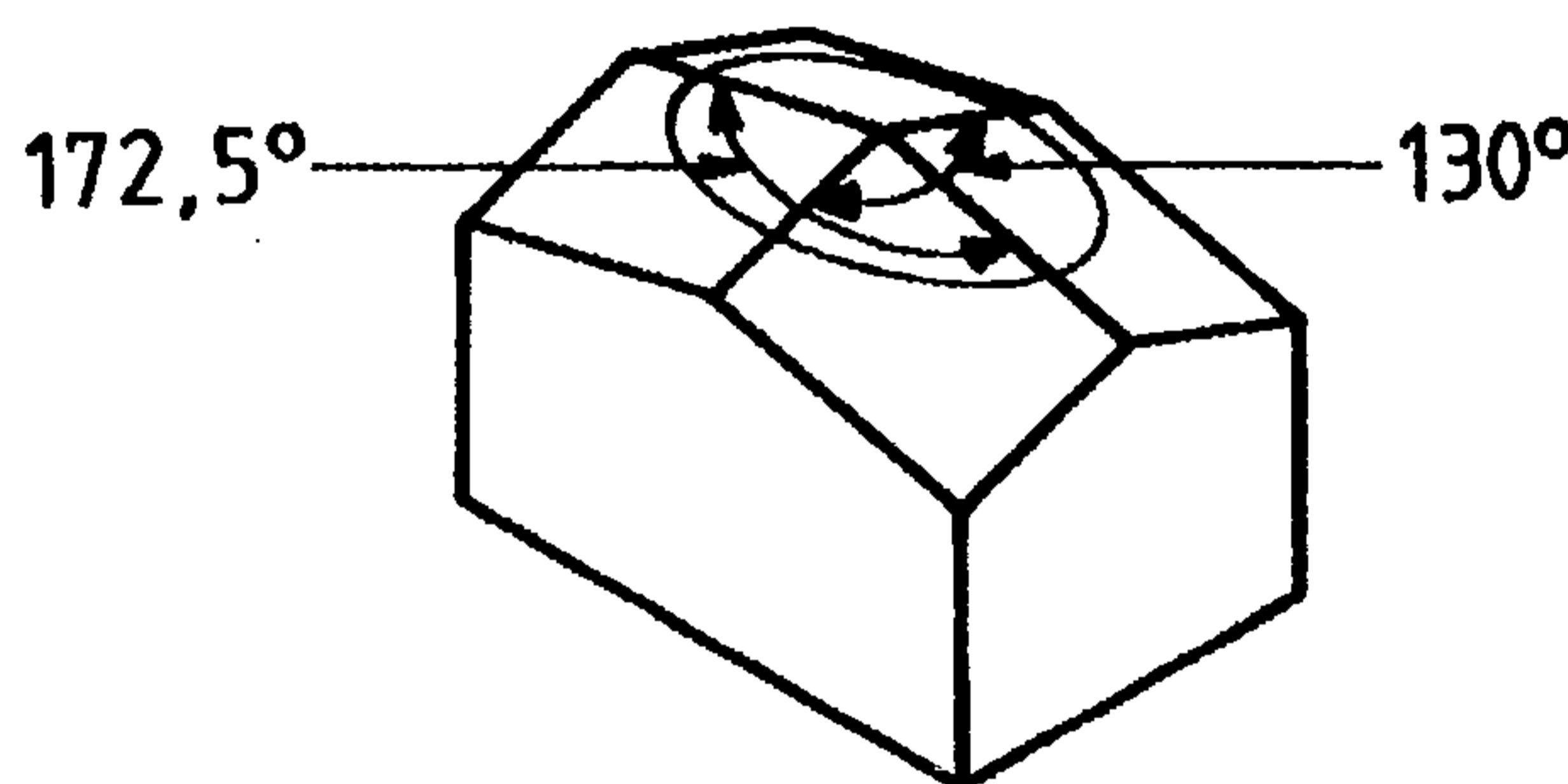
Figure 2 — Knoop indenter
