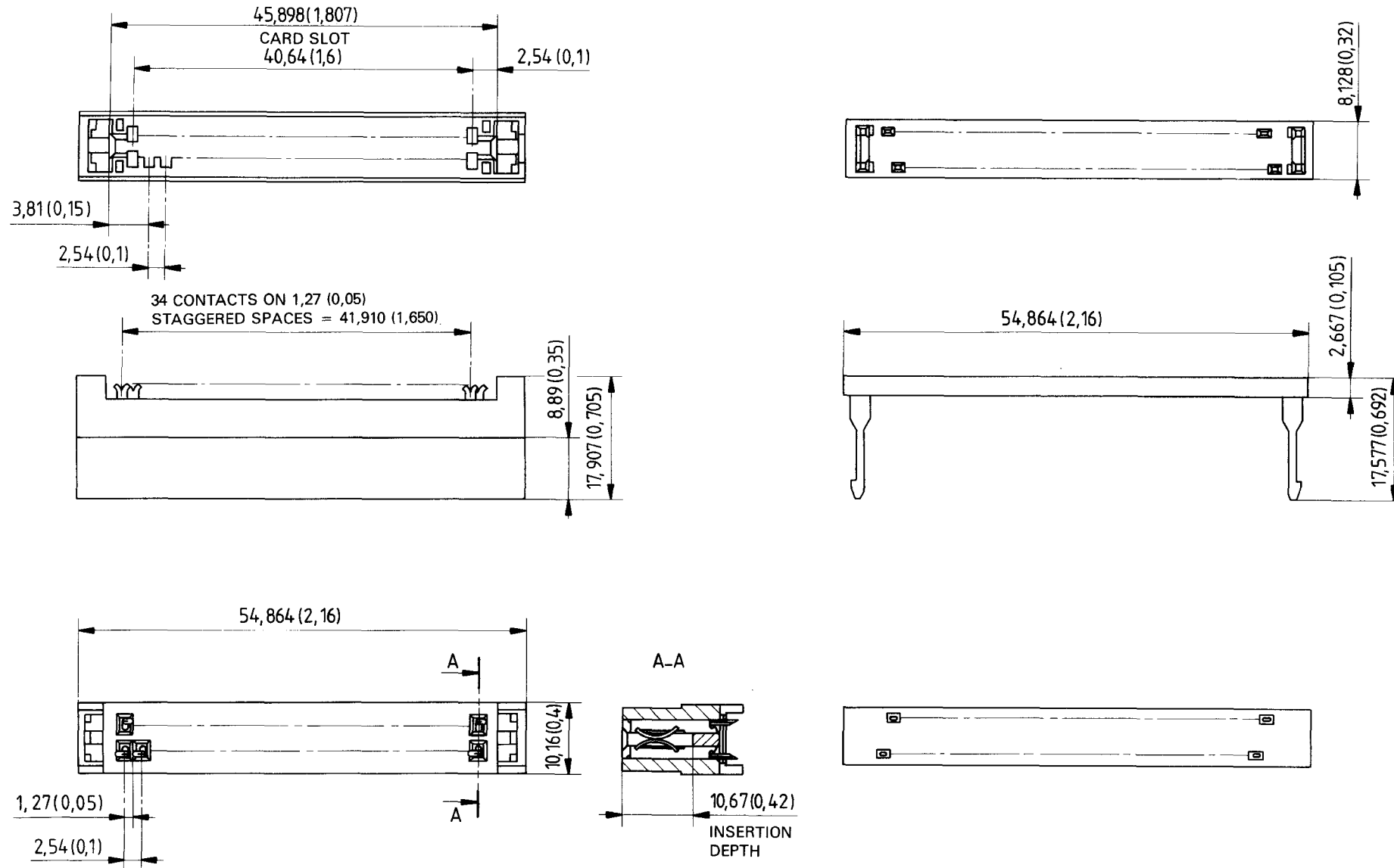
Figure 20 — Signal interface cable connector for 130 mm (5,25 in) drive
