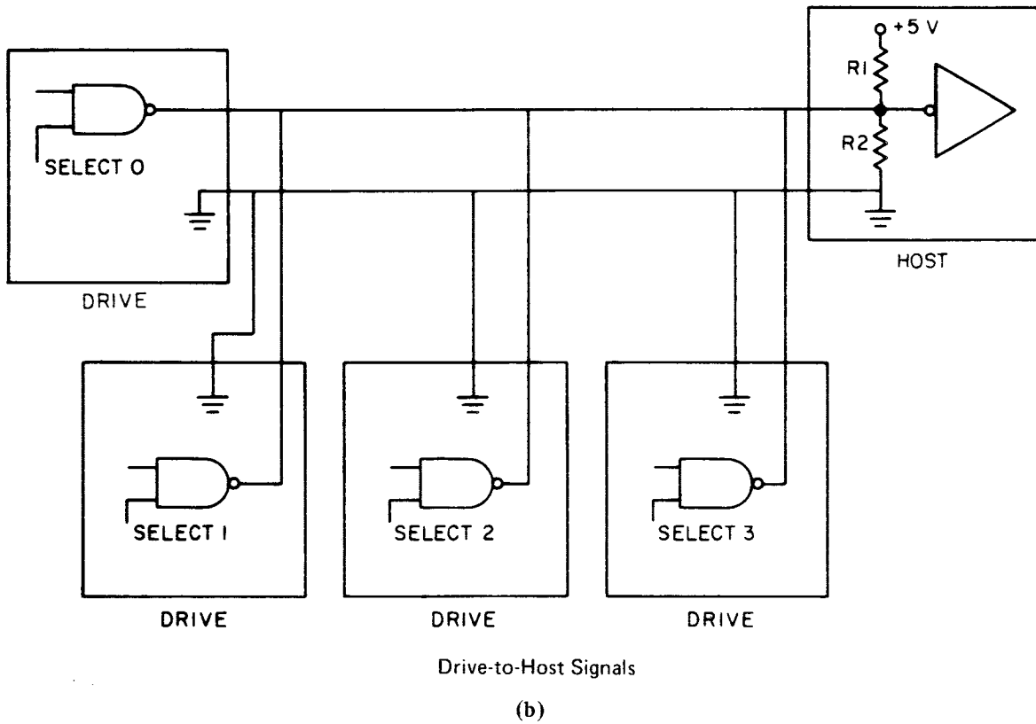
Figure 15 — Interface interconnect circuit scheme
