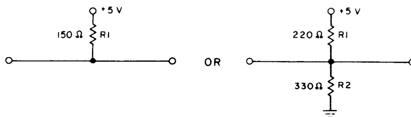
Figure 16 – Resistive termination networks
