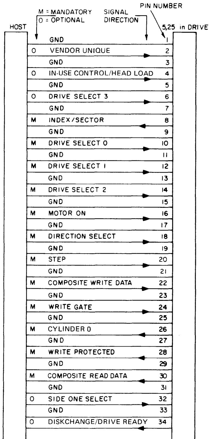
Figure 2 — 130 mm (5,25 in) cartridge drive signals
