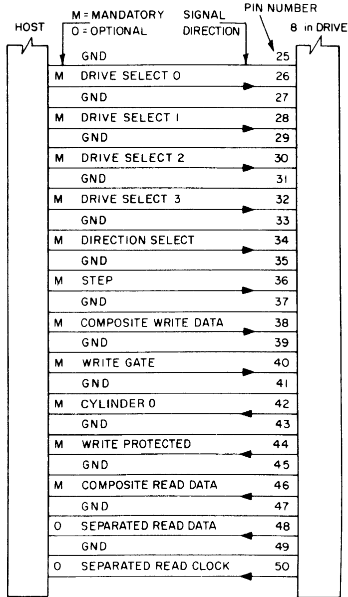
Figure 1 — 200 mm (8 in) cartridge drive signals
