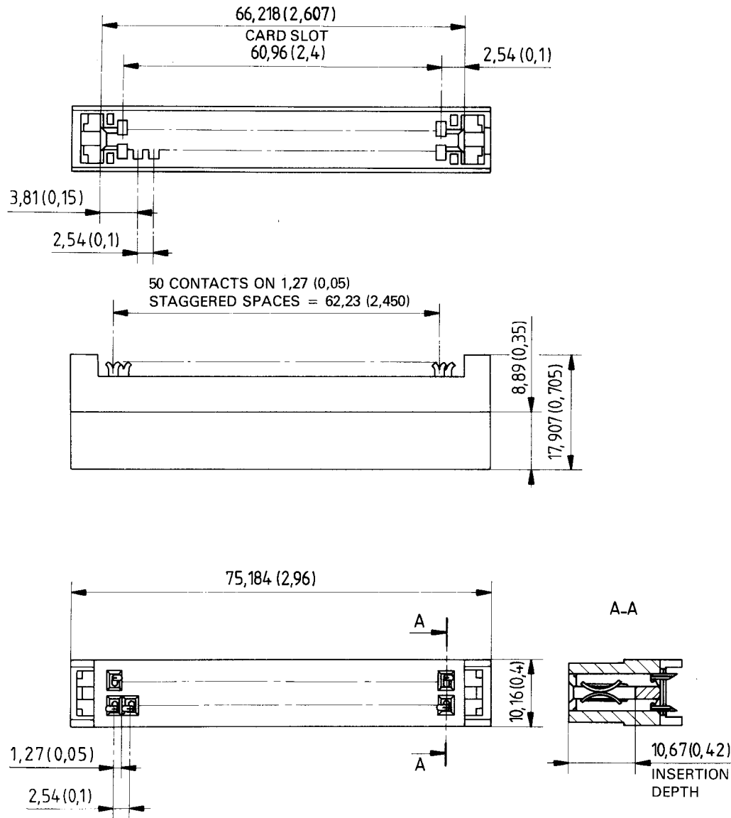
Figure 19 — Signal interface cable connector for 200 mm (8 in) drive
