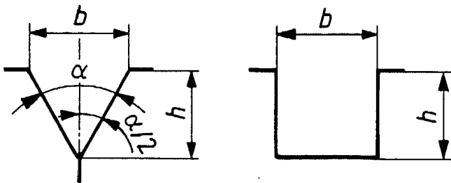
"V" type notch (only to be used when h < 0,5 mm)
