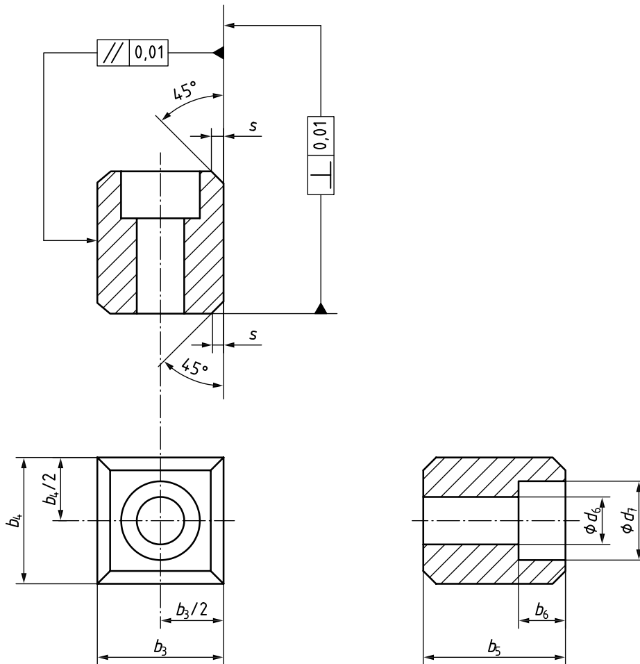
Figure 3 — Tenon dimensions for spindle noses of forms J and JF
