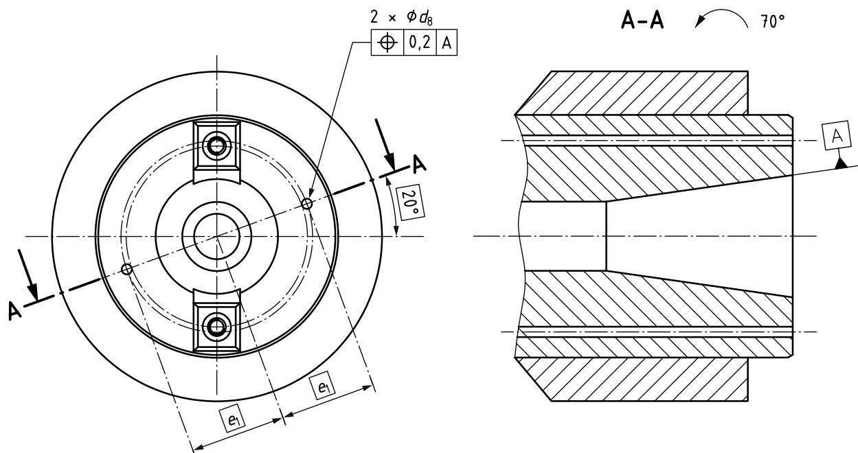
Figure 2 — 7/24 taper spindle noses of form JF for tool shank of form JF
