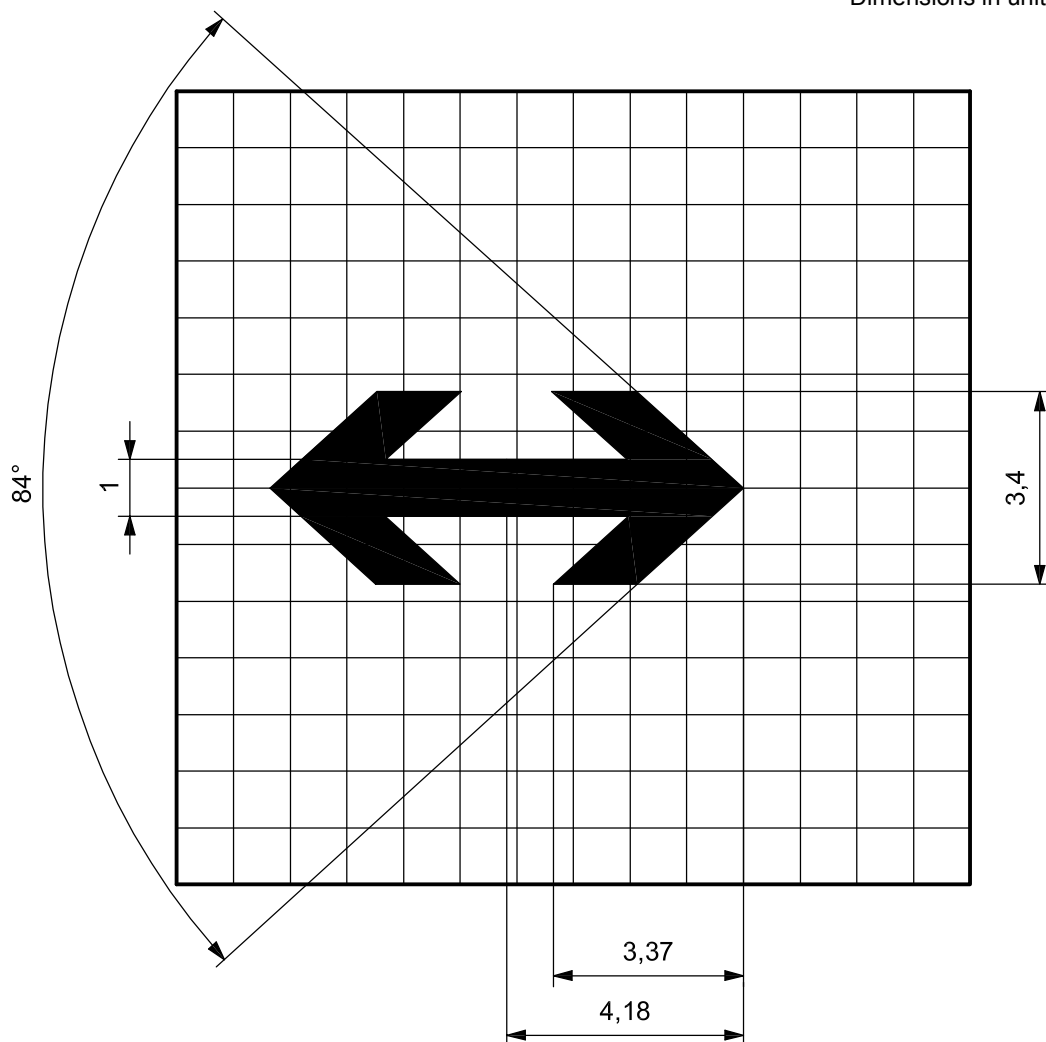
Figure D.24 — Arrow representing the idea of keeping a safe distance away from hazard
