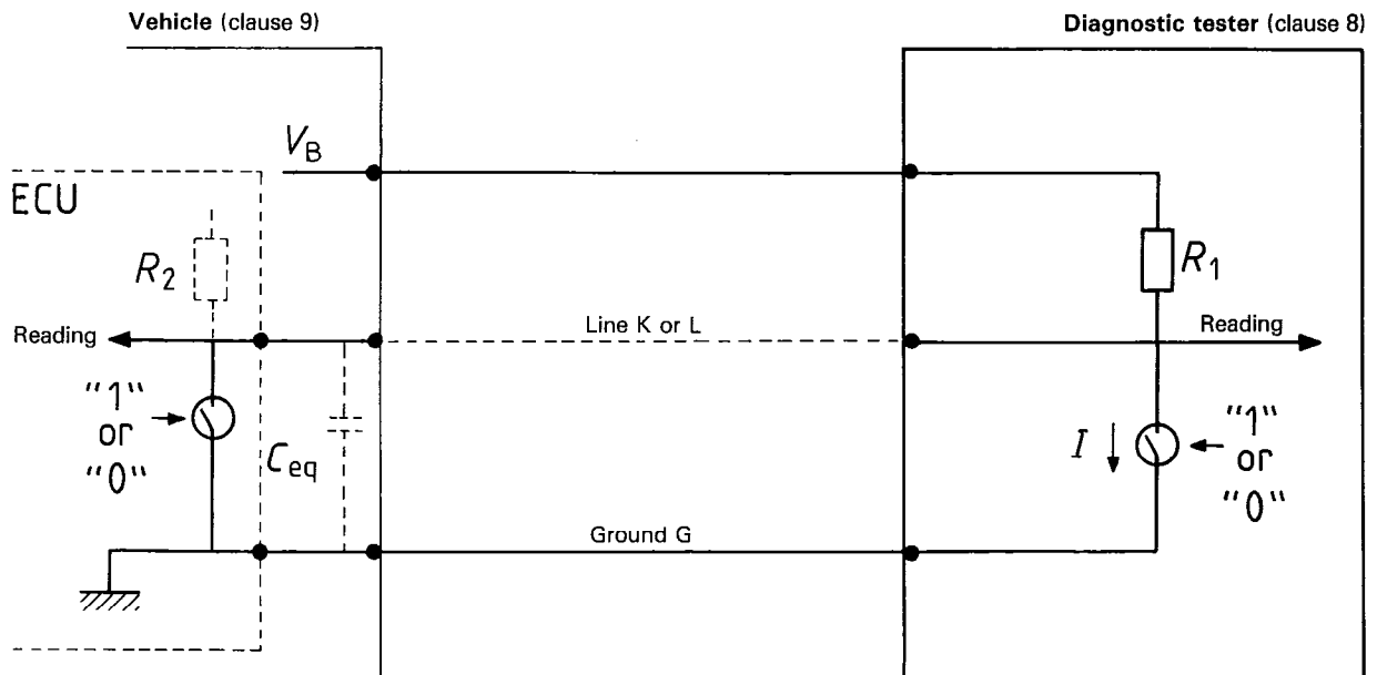
Figure 5 — Communication — Schematics
