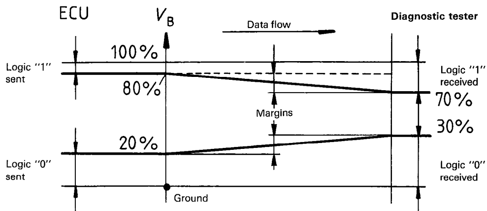
Figure 4 — Signal voltage levels, data flow from ECU to the diagnostic tester: worst-case values
