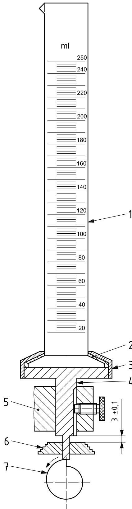
Figure 1 — Bulk density apparatus
