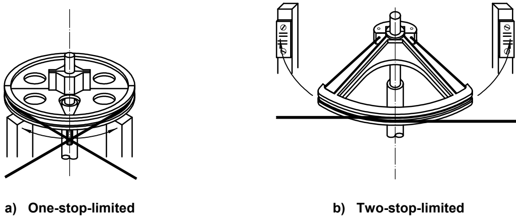
Figure 7 — Steering-arm rotation
