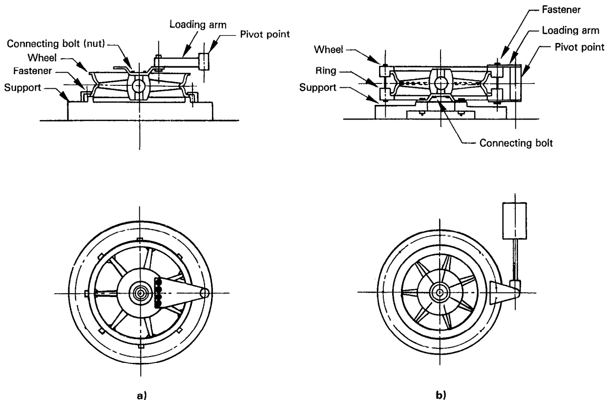
Figure 4 — Model equipment for torsion test
