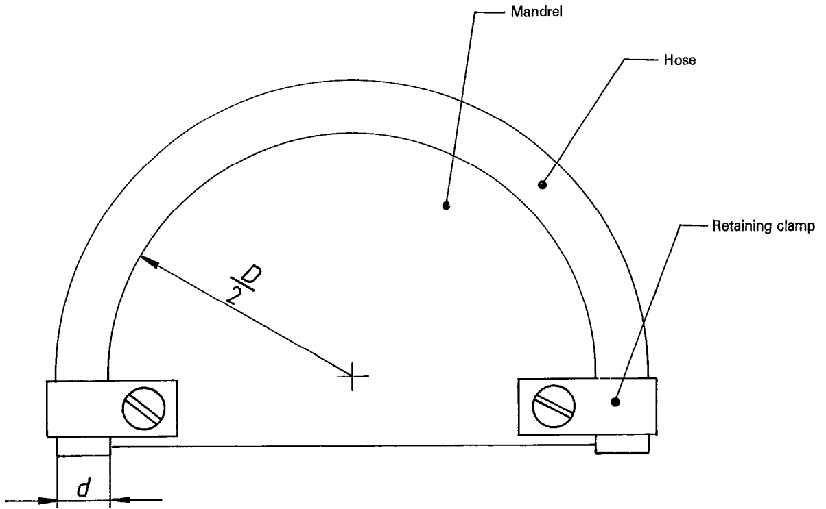
Figure 1 — Arrangement for mounting hose on mandrel for Method 1
