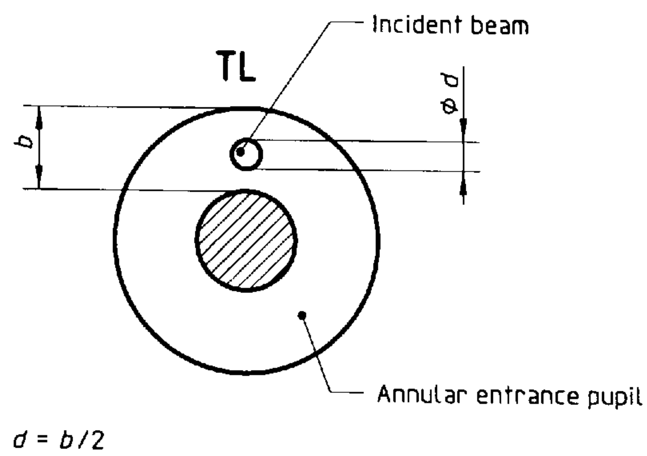
c) Diameter of the incident beam
