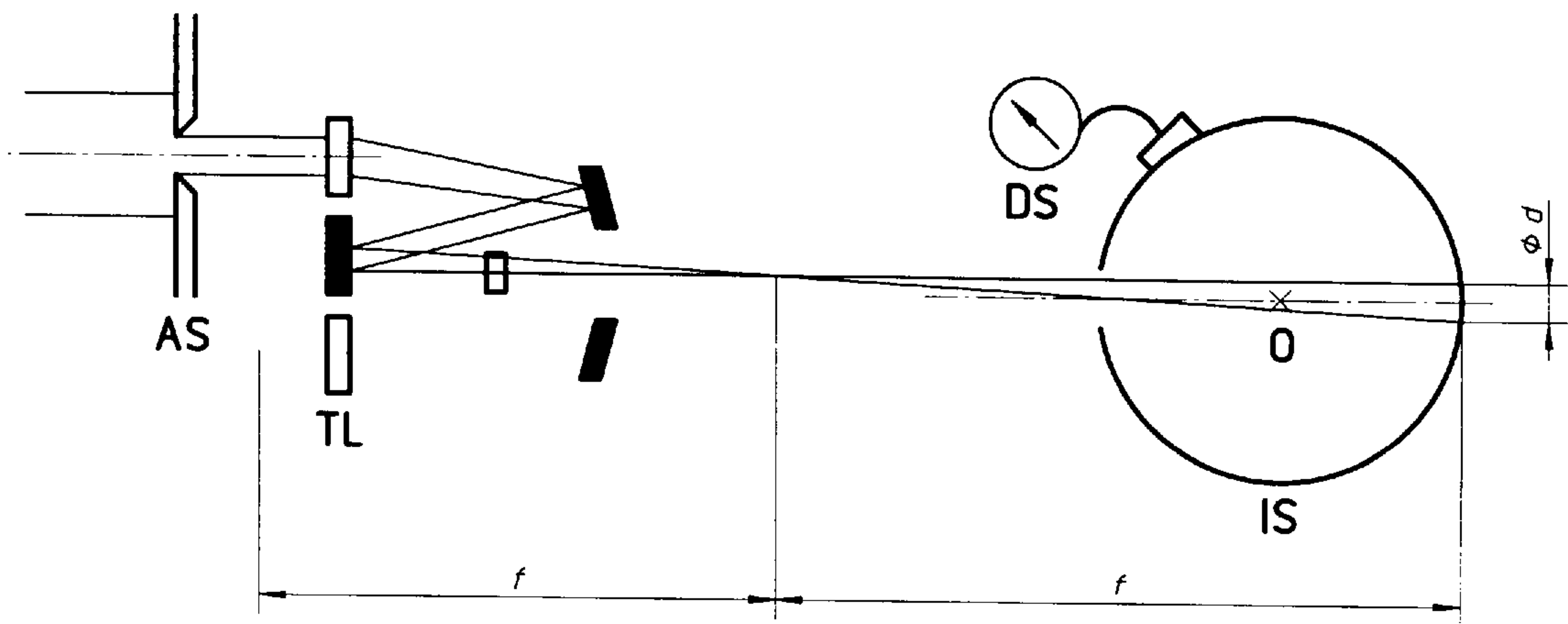
b) Measuring transmitted radiant flux
