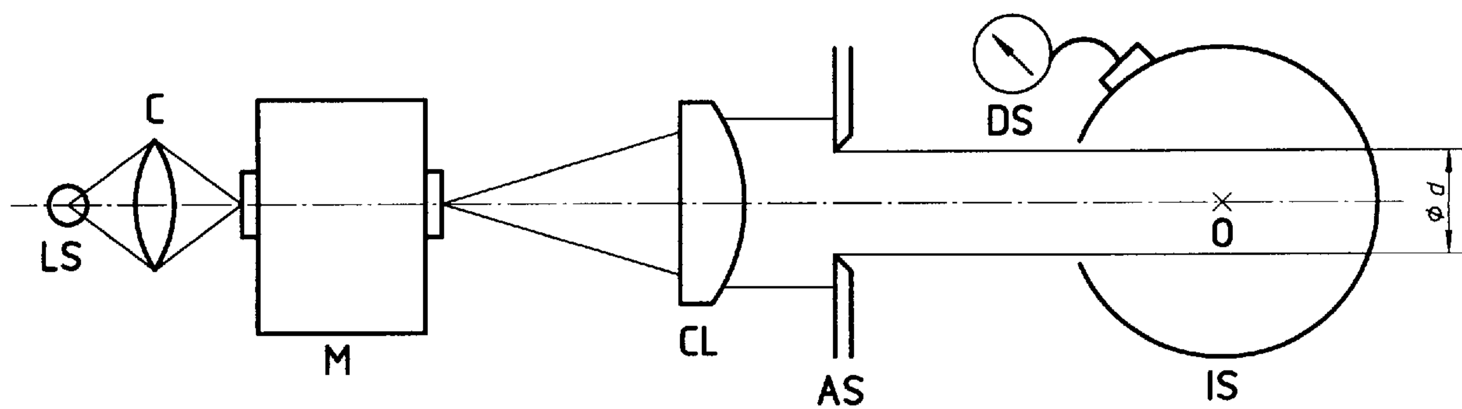
a) Using a collimator lens
