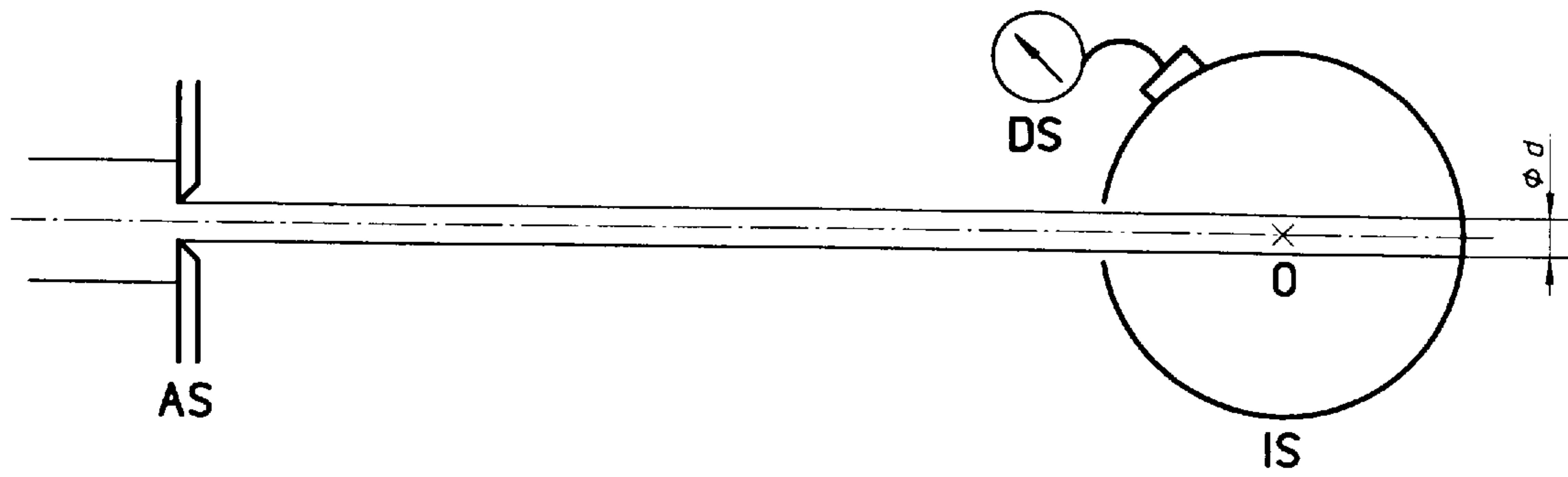
a) Measuring incident radiant flux
