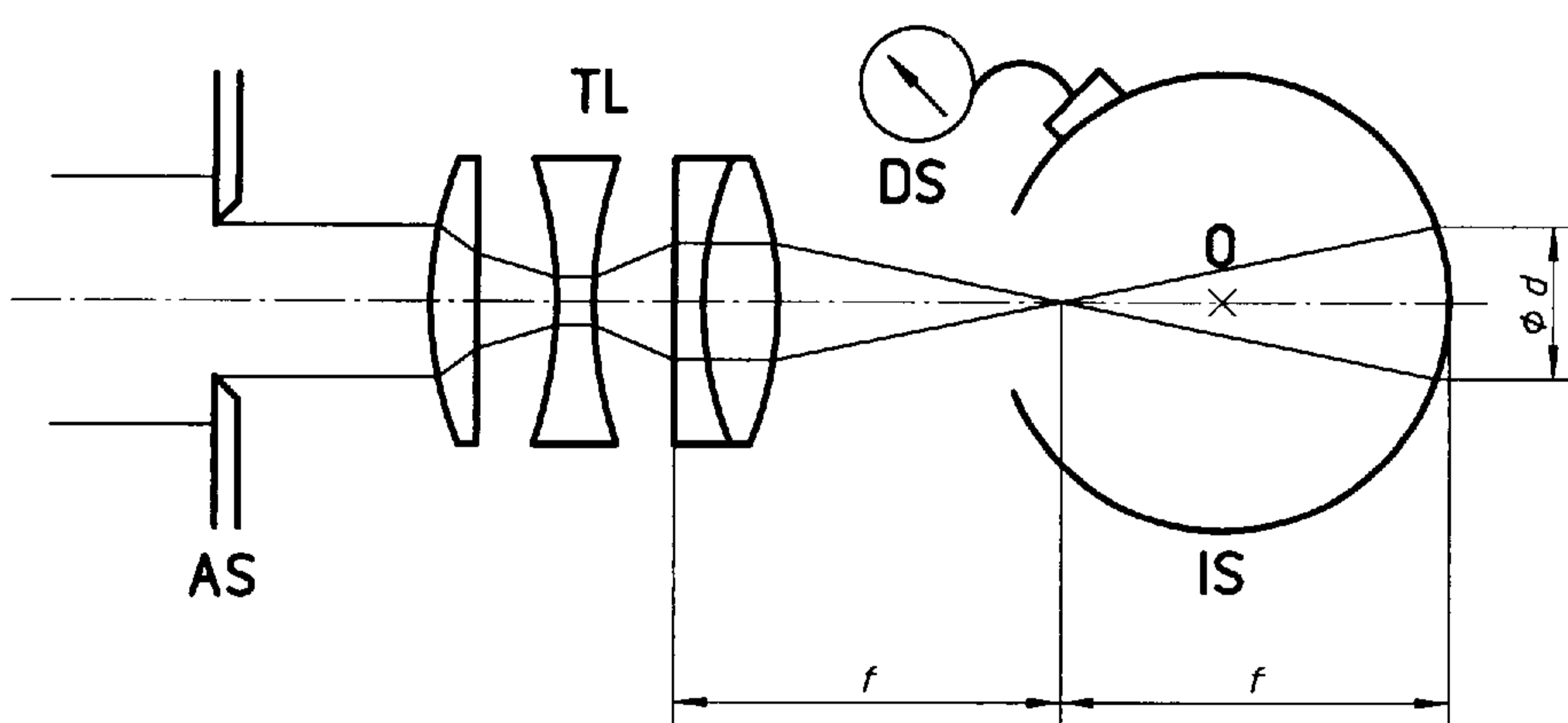
b) Measuring transmitted radiant flux
