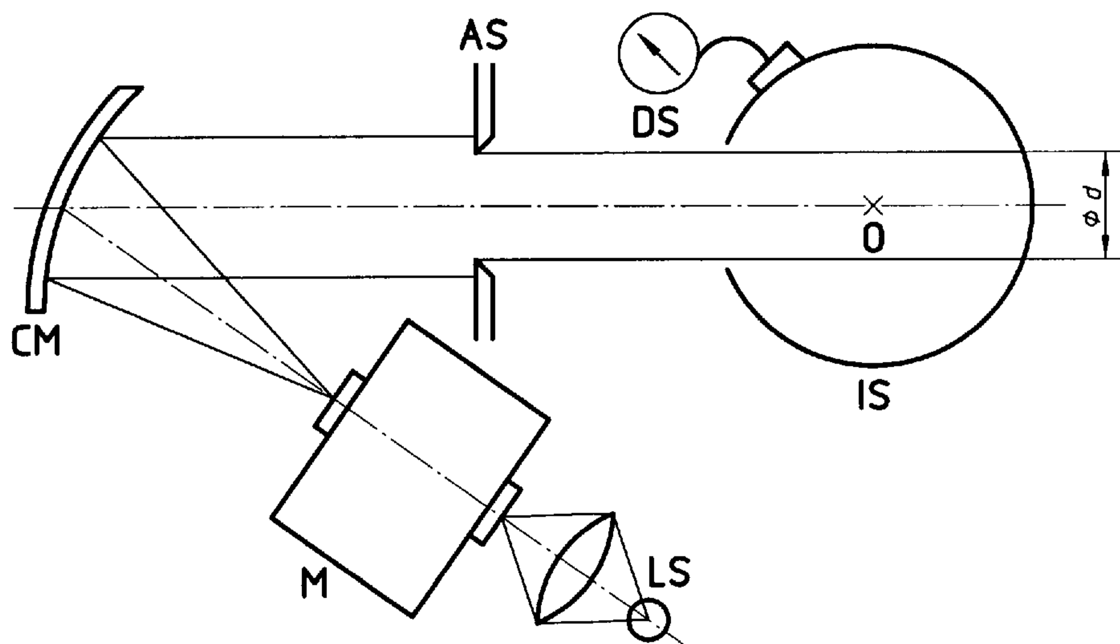
b) Using an off-axis paraboloid mirror collimator
