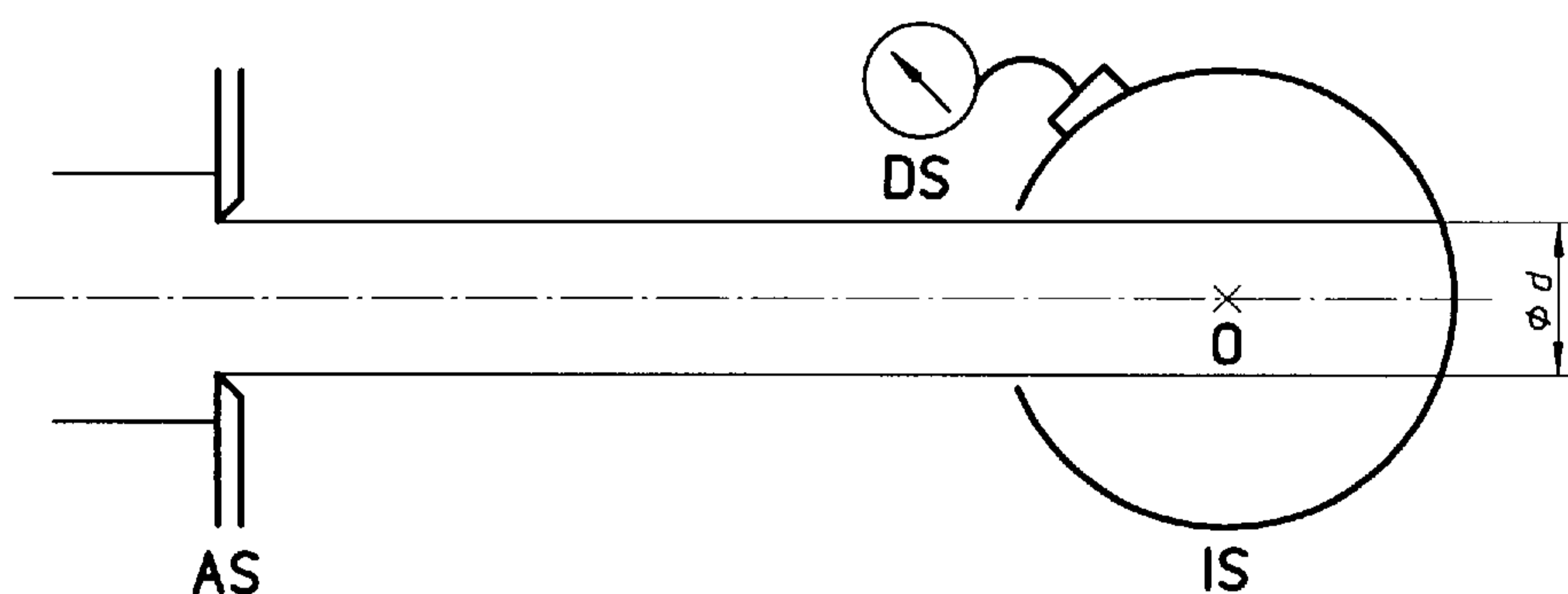
a) Measuring incident radiant flux
