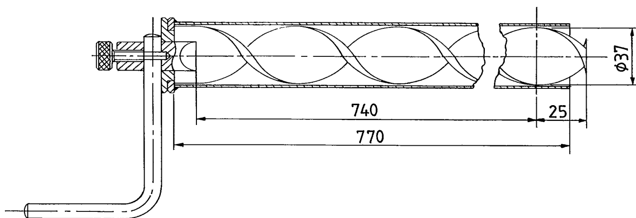
Figure 9 — Shuttered sampling auger (Archimedes) (see 4.1.2)
