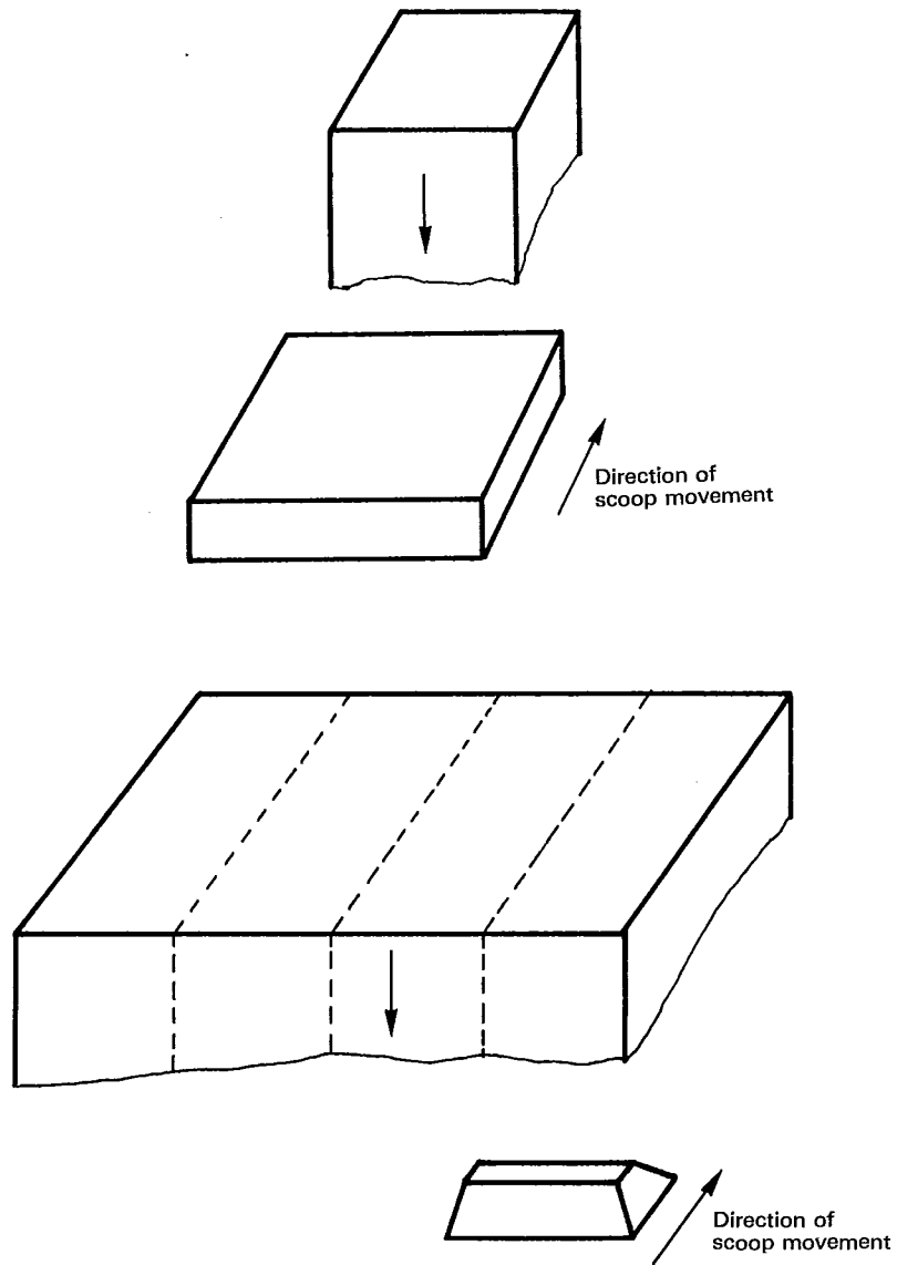
Figure 24 — Cross-sectional samples of a falling stream (see 5.6.4.3)
