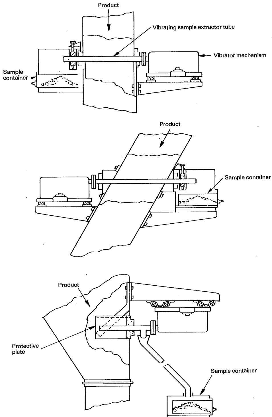
Figure 21 — Continuous automatic samplers (see 4.1.4)
