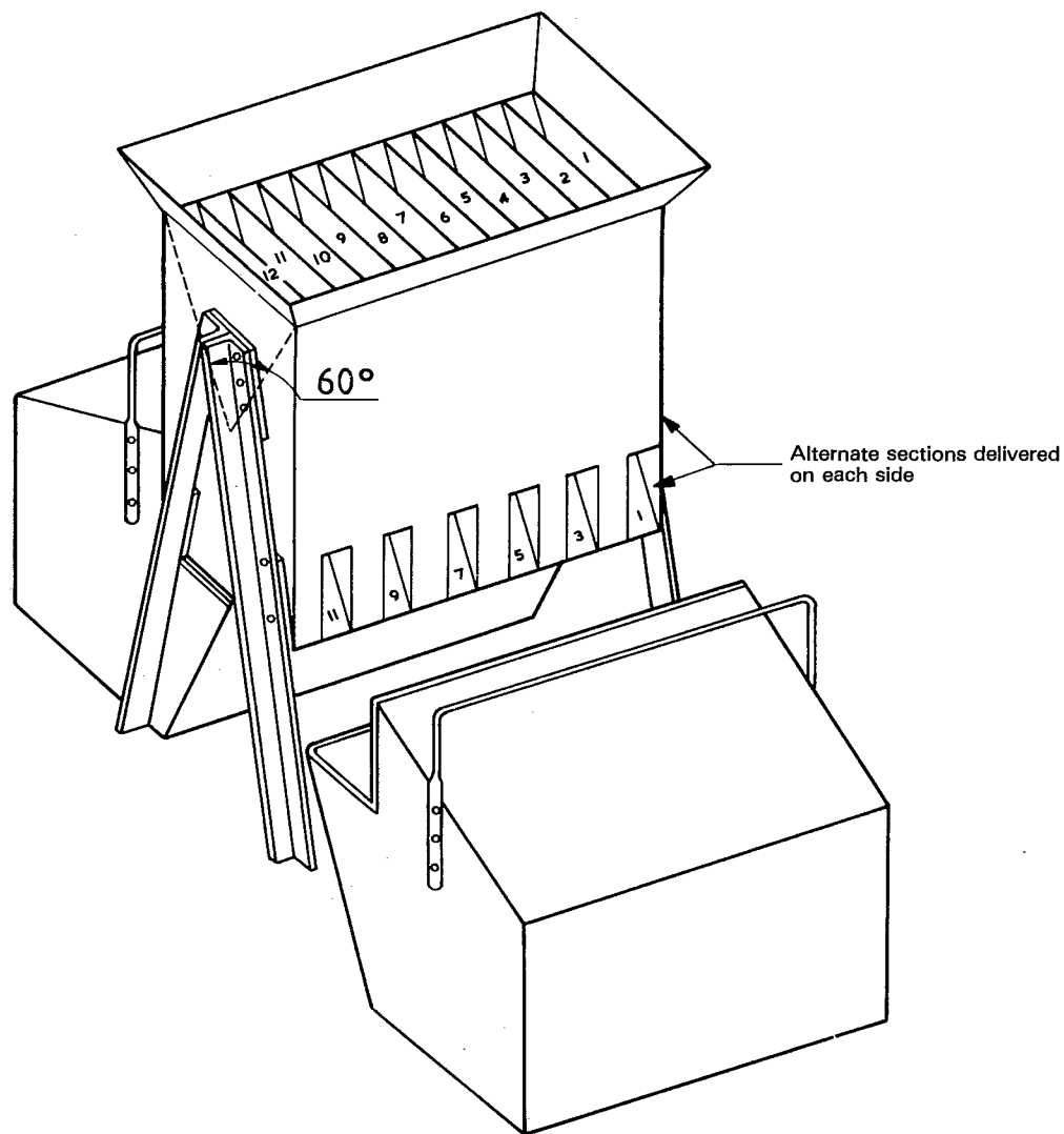
Figure 14 — Riffle sample divider (see 4.1.3)
