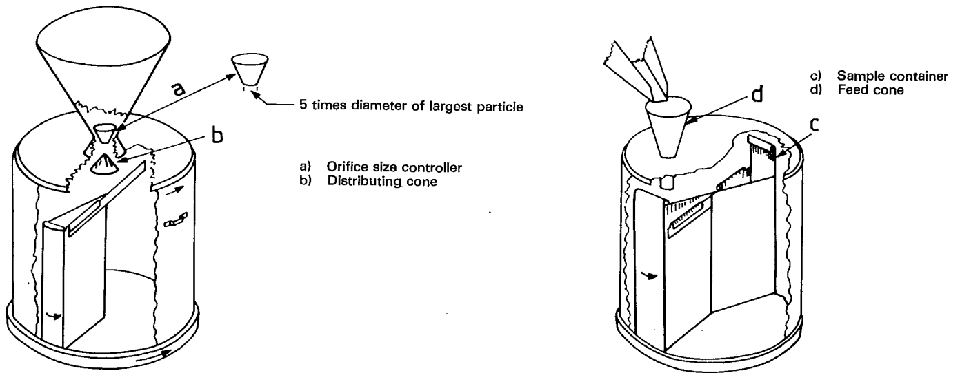
Figure 17 — Rotary sample dividers (see 4.1.3)
