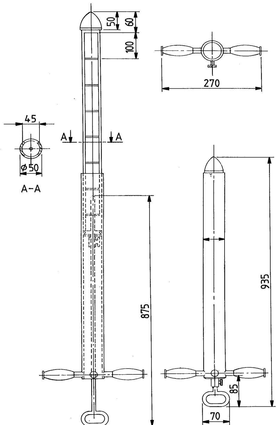
Figure 5 — Closable sampling spear
