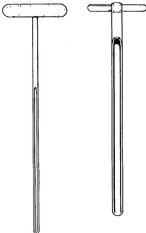
Figure 4 — Further designs of open-end sampling spears
