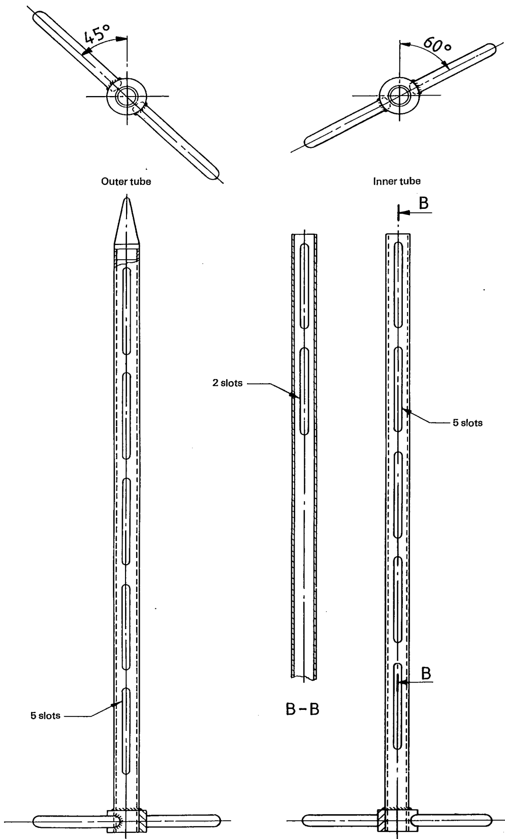
Figure 6 — Shuttered sampling spear
