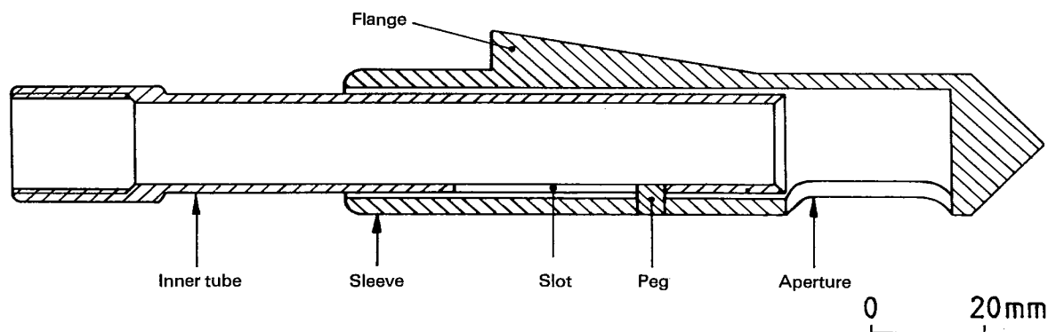
Figure 12 — Spear for suction sampling device (see 4.1.2)
