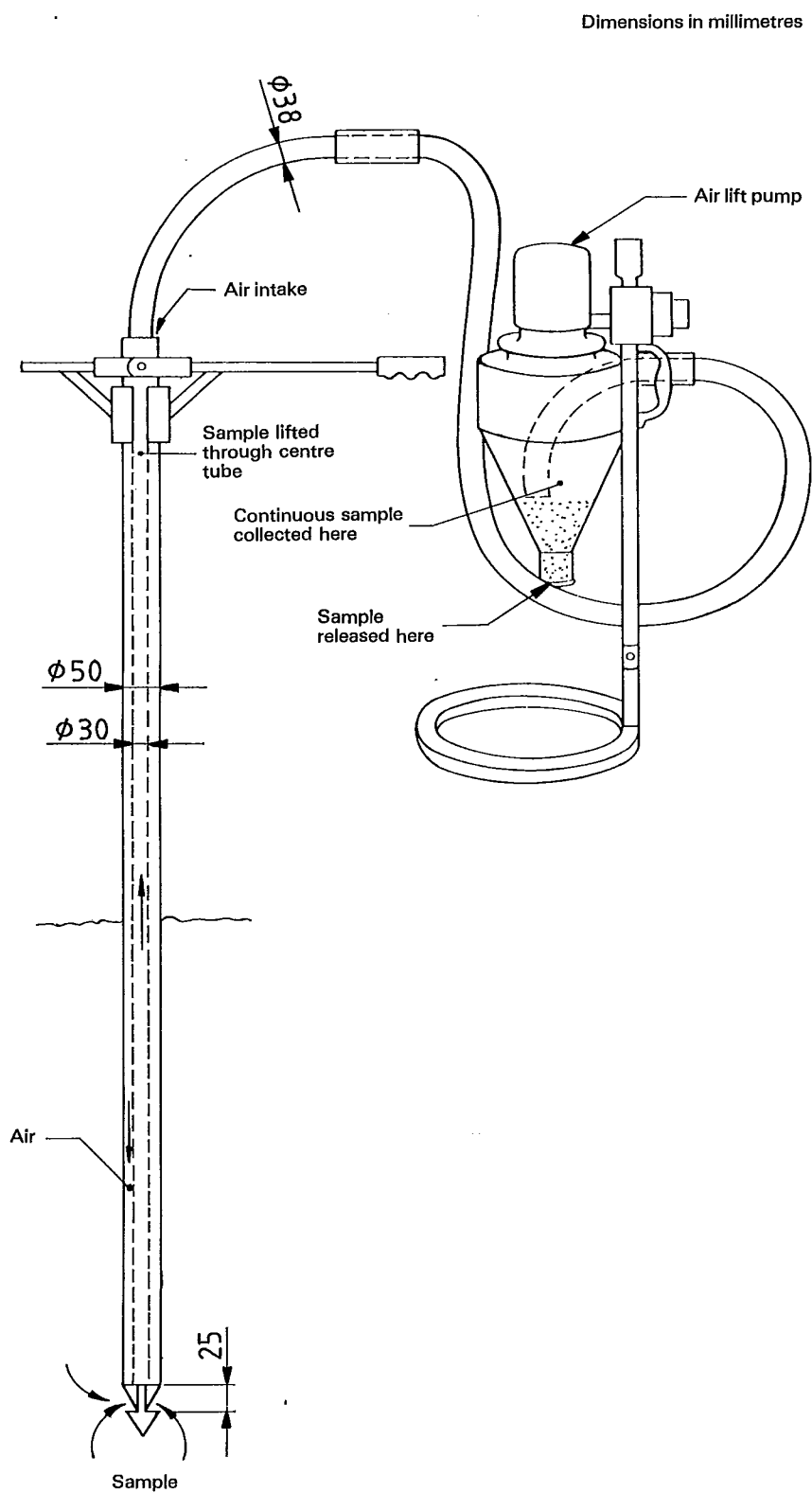
Figure 10 — Pneumatic probe sampler (see 4.1.2)
