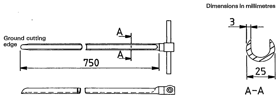
Figure 2 — Open-end sampling spear
