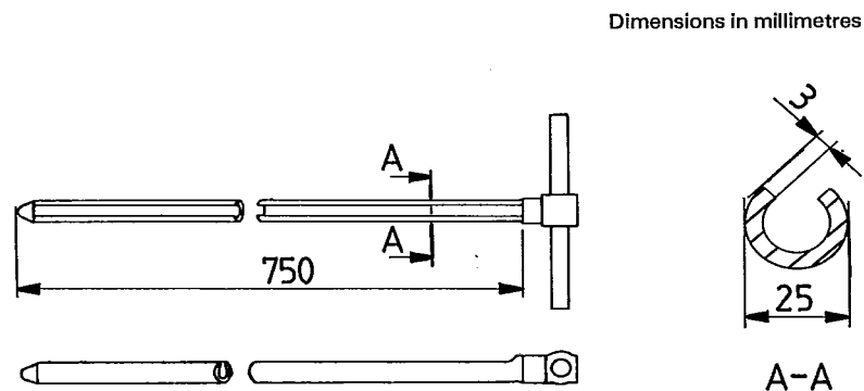
Figure 3 — Closed-end sampling spear
