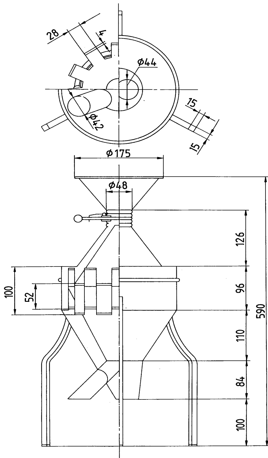
Figure 15b — Diagram of a typical conical divider (see ISO 607)
