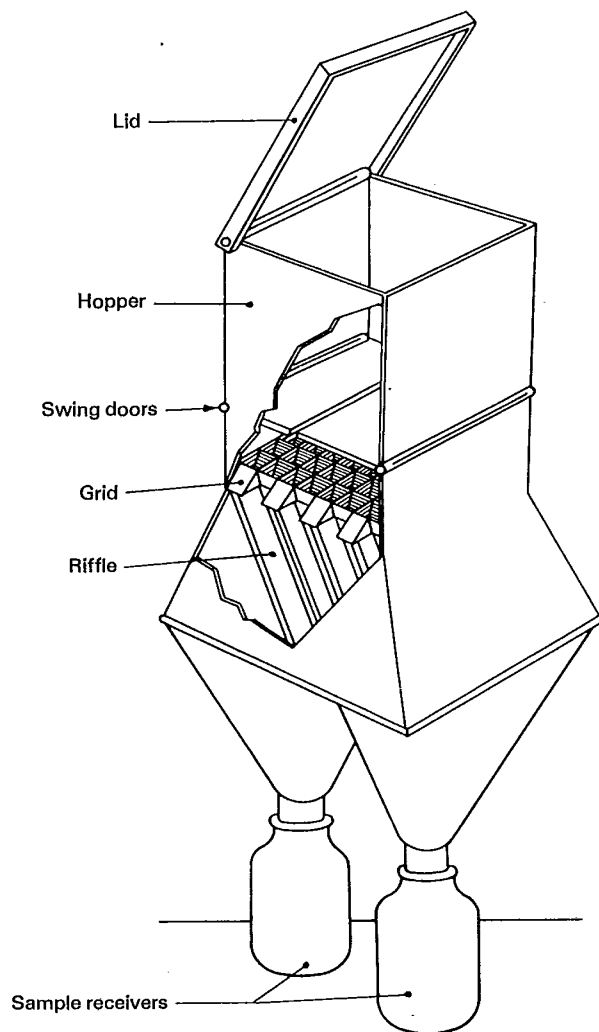
Figure 16 — Grid-type sample divider (see 4.1.3)
