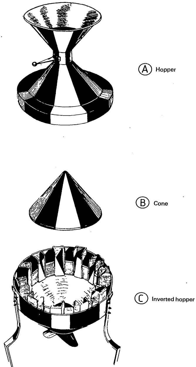
Figure 15a — Exploded view of a typical conical divider (see ISO 607)
