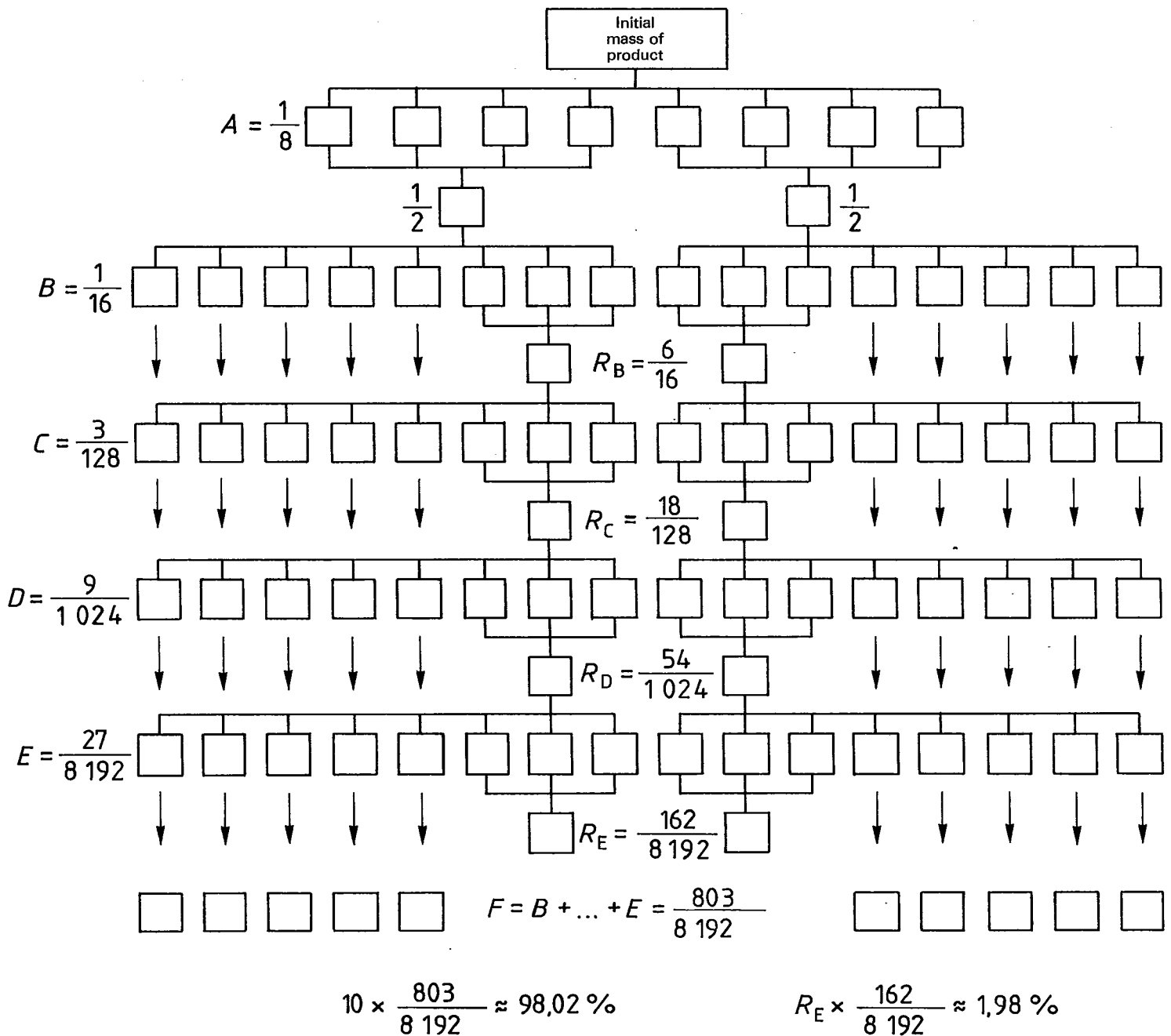
Figure 25 — Obtaining 10 equal representative fractions with a divider into 8 (see 5.6.6.1)
