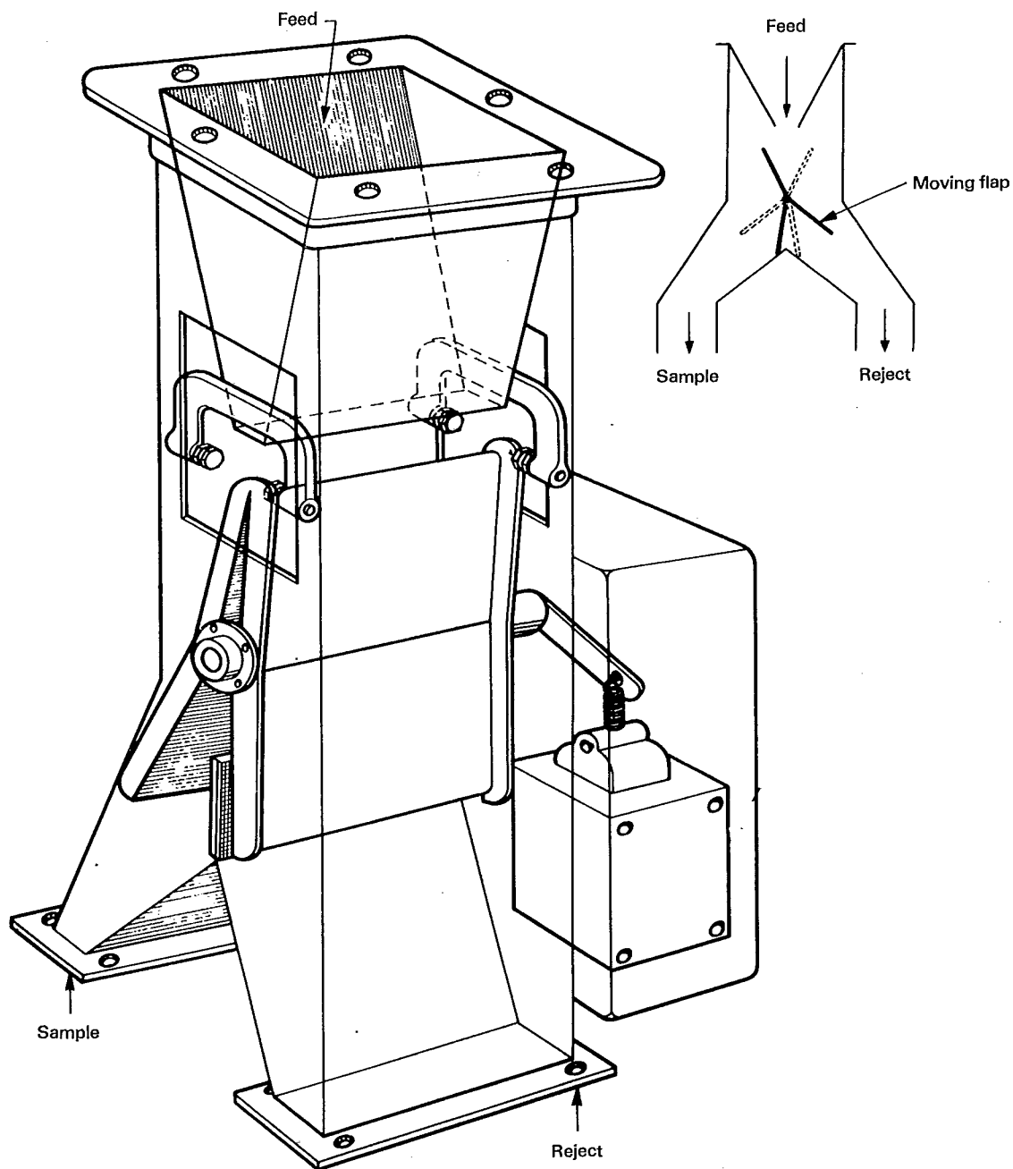
Figure 19 — Moving-flap sample divider (see 4.1.3)
