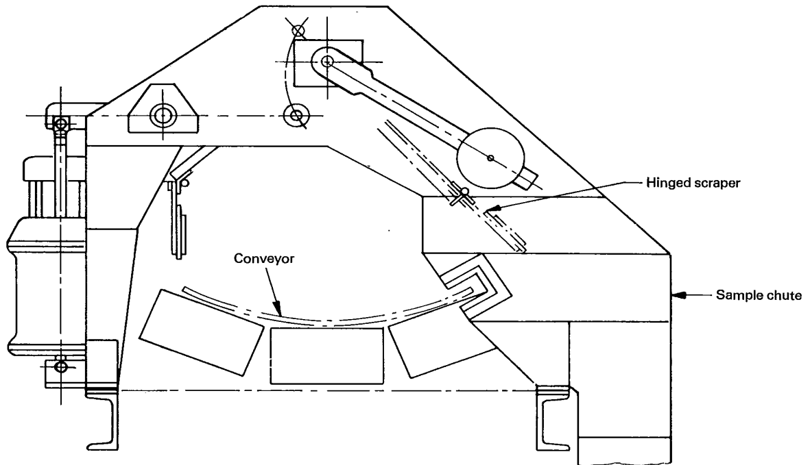
Figure 22 — Automatic sampler for belt conveyor (see 4.1.4)
