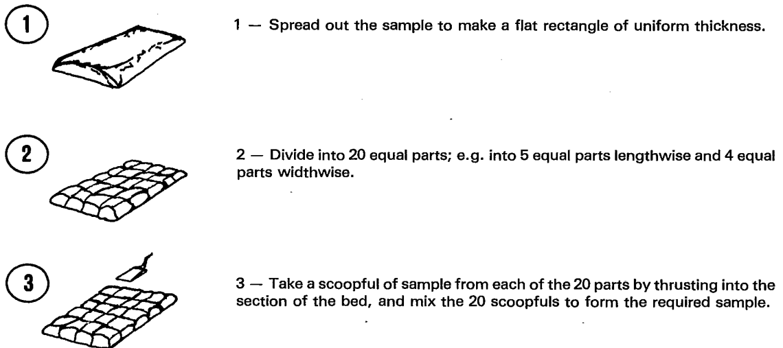
Figure 23 — Alternate division procedure (see 5.6.4.2)
