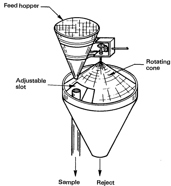
Figure 18 — Double-cone sample divider (see 4.1.3)
