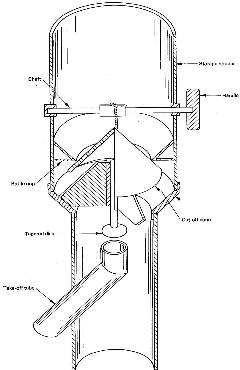
Figure 13 — Granular material sampler (see 4.1.3)
