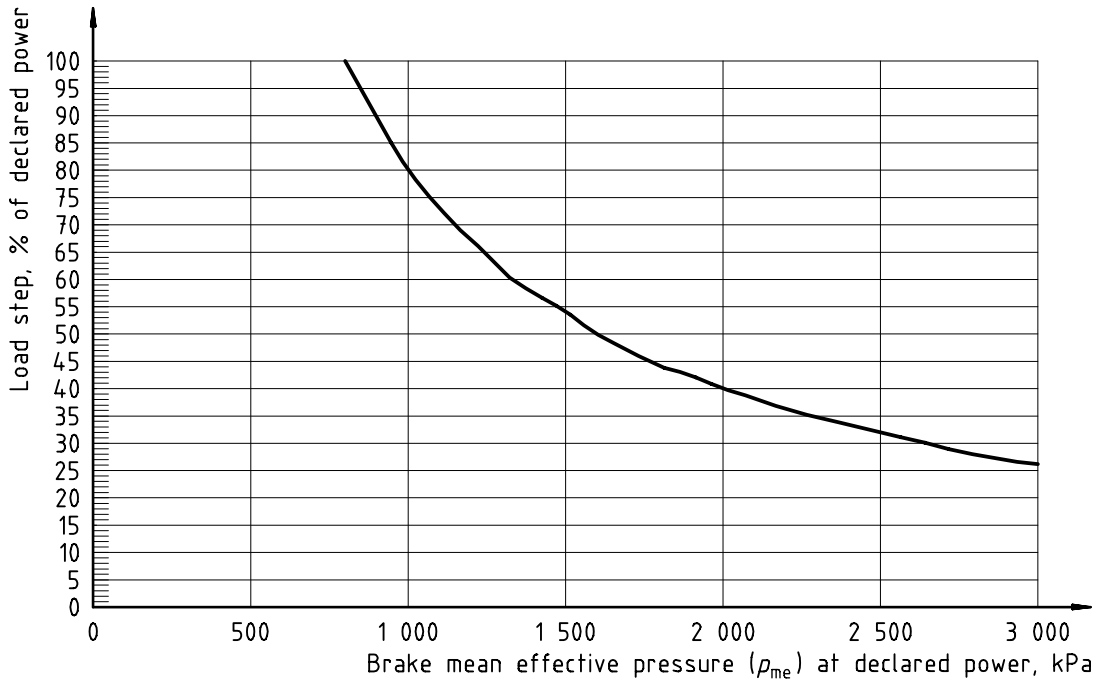
Figure B.1 — Load step for four-stroke engines
