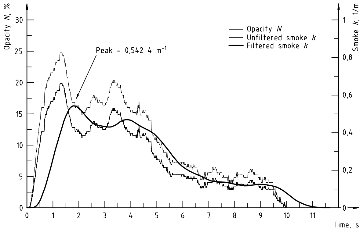
Figure D.3 — Traces of measured opacity N , of k for unfiltered smoke and of k for filtered smoke
