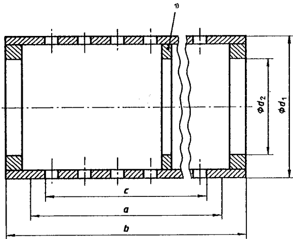
1) The number of stiffening ribs depends on the construction, length and diameter of the beam.
