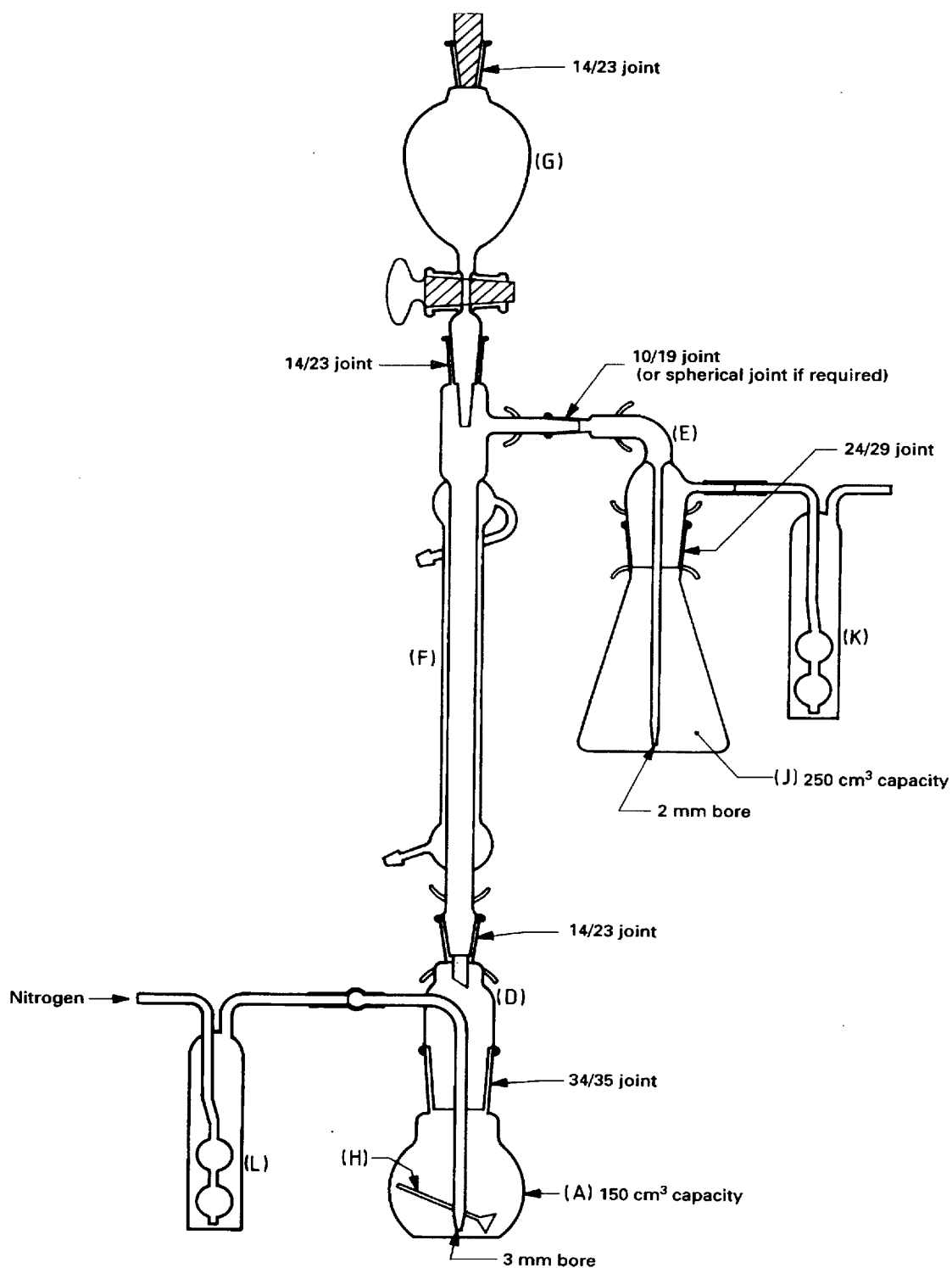
Figure 2 — Typical apparatus for the evolution and absorption of hydrogen sulfide
