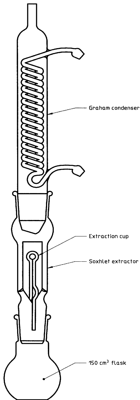
Figure 1 — Extraction apparatus
