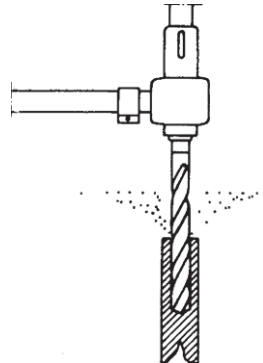
Figure C.2 — Oil-hole drill
