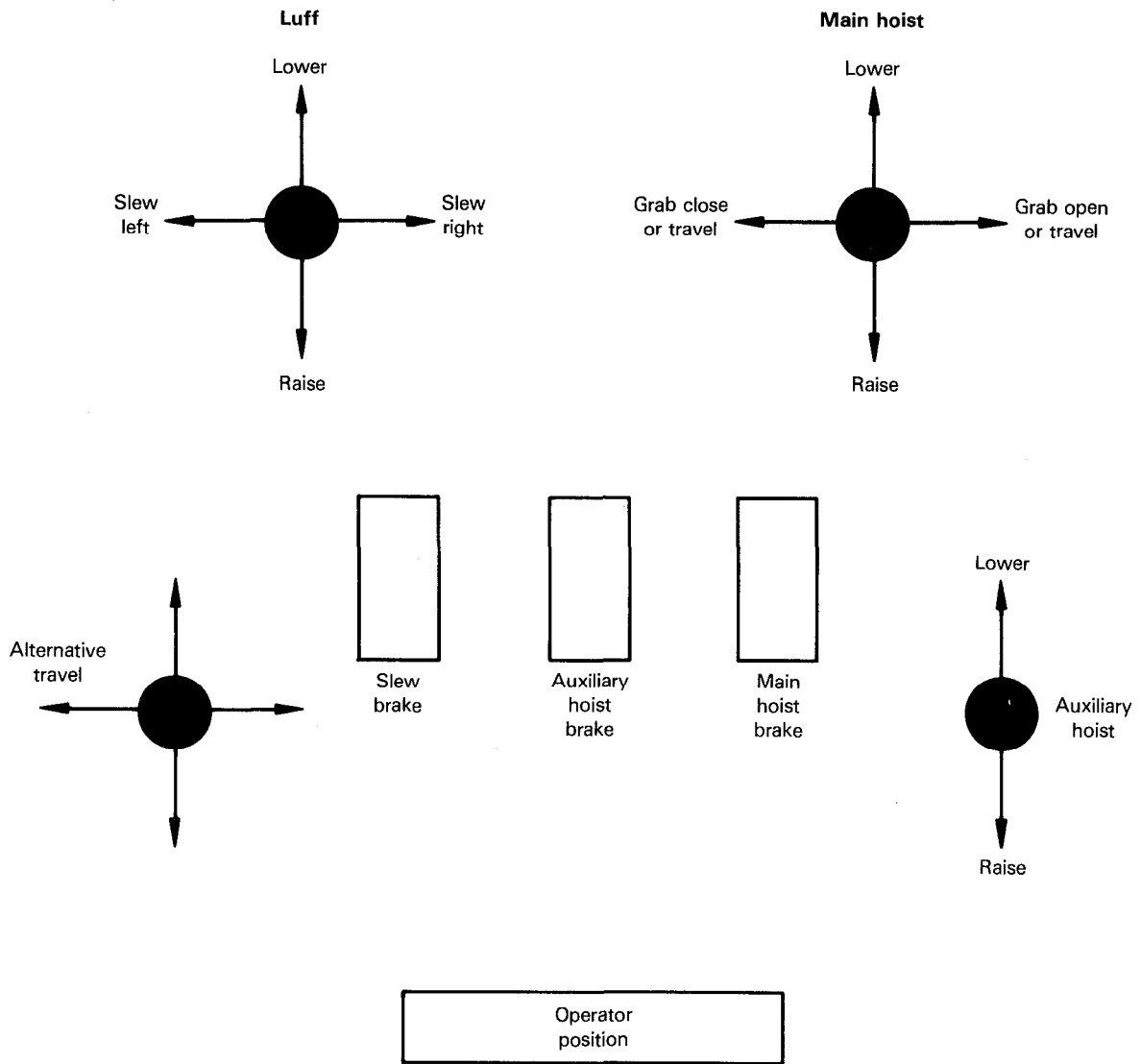
Figure 2 – Crane control diagram for crane fitted with a fixed or articulated jib and multi-directional controls
