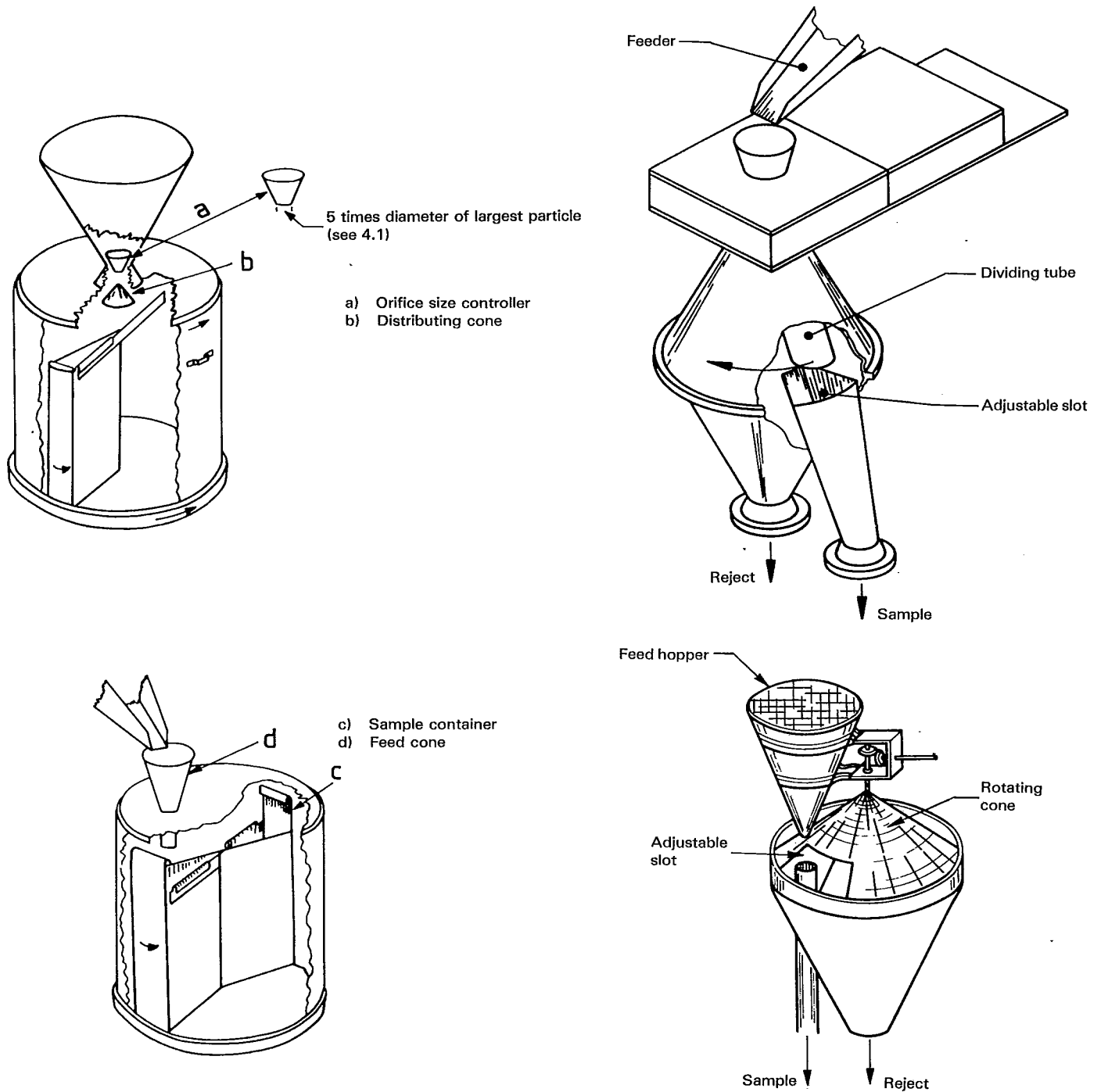
Figure B.1 — Rotating sample dividers
