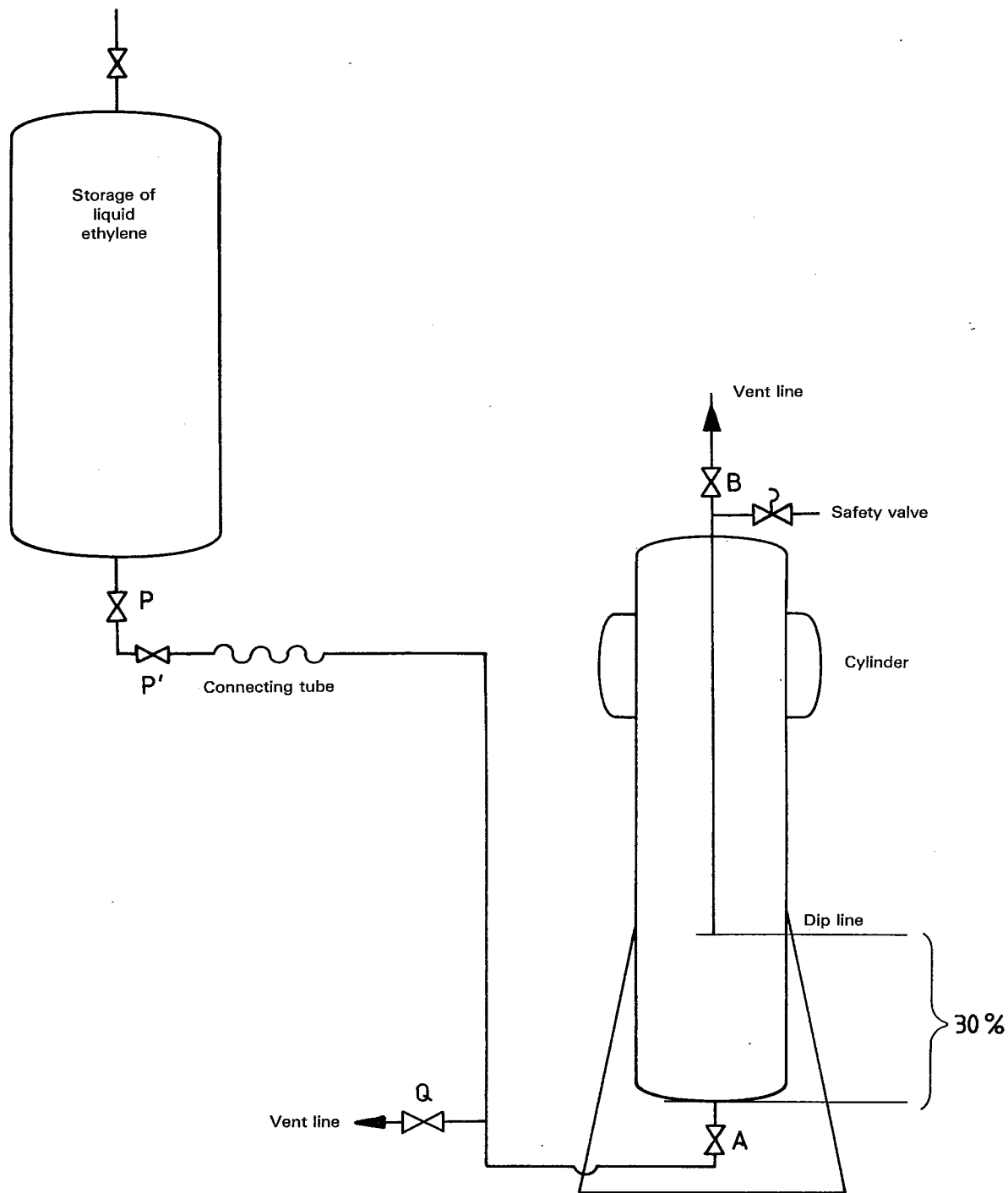
Figure 1 — Sampling apparatus No. 1 for liquid ethylene
