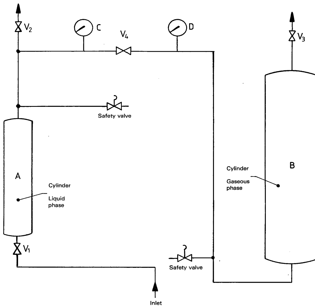
Figure 2 — Sampling apparatus No. 2 for liquid ethylene
