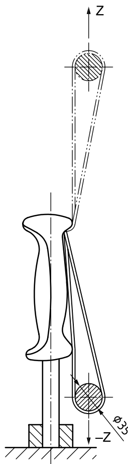
Figure 5 — Test arrangement for the strap
