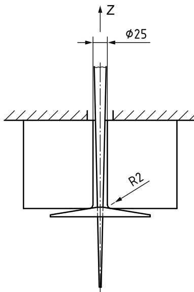
Figure 9 — Test arrangement for the basket fixing in the direction of the tensile force
