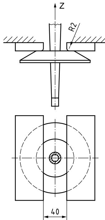
Figure 10 — Gap for testing the basket
