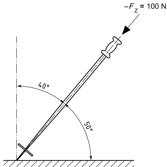
Figure 11 — Test of ice gripping power
