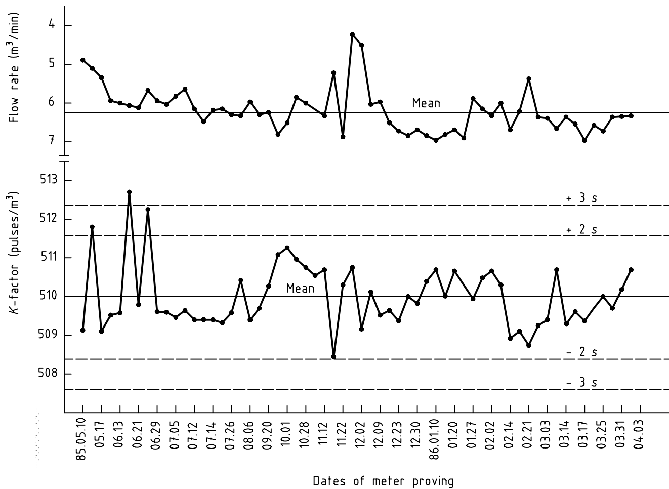
Figure 8 — Example of control chart
