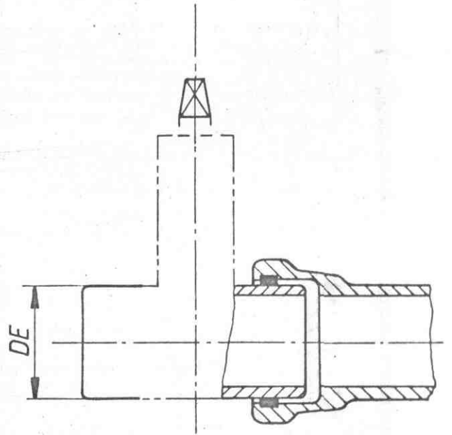
Figure 2 — Spigot end valve
