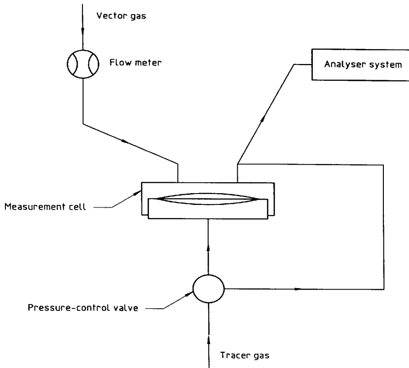
Figure 1 — Apparatus (schematic diagram)
