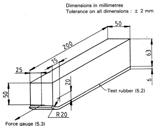
Figure 1 — Test block
