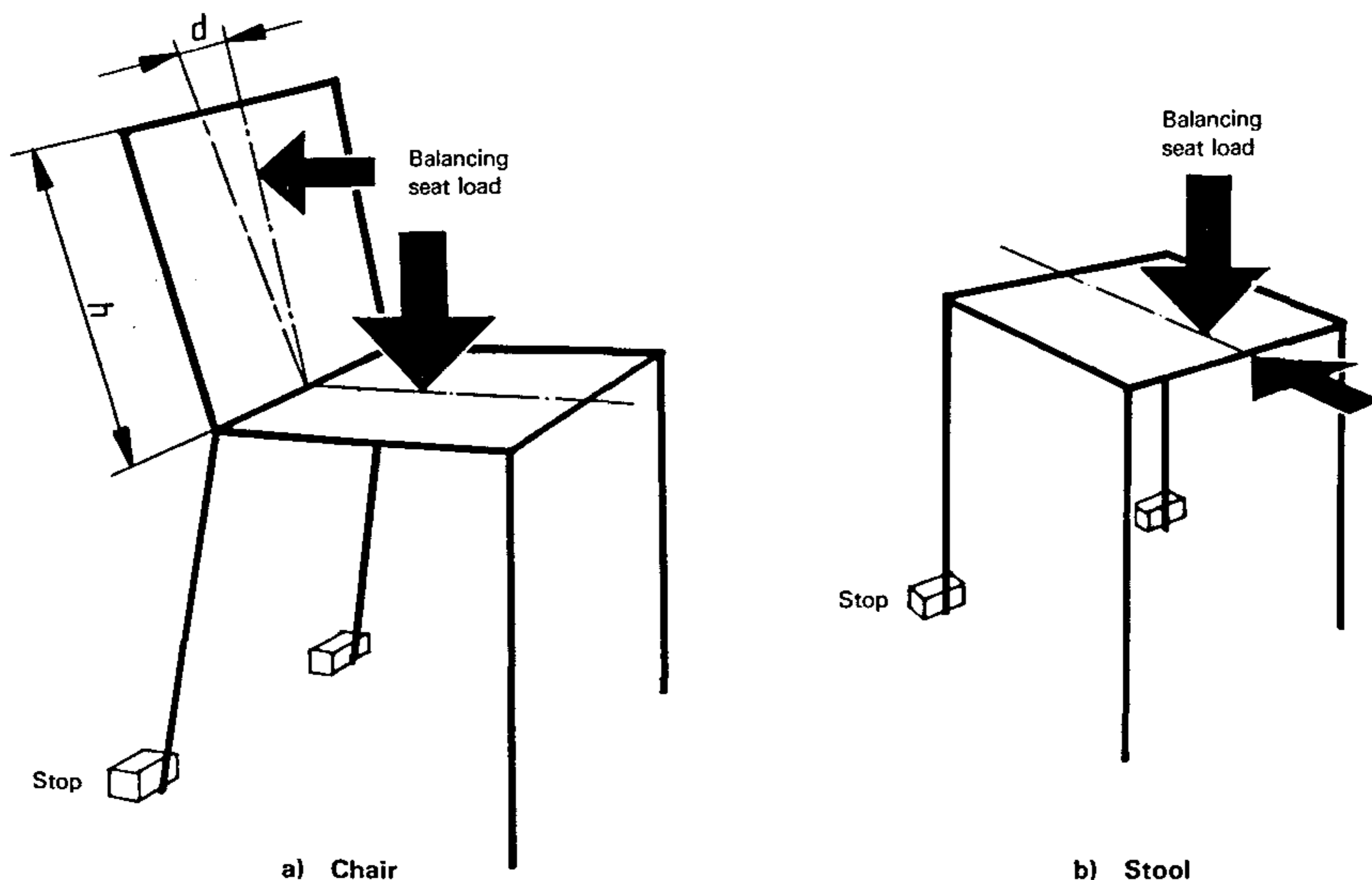
Figure 2 — Back static load test
