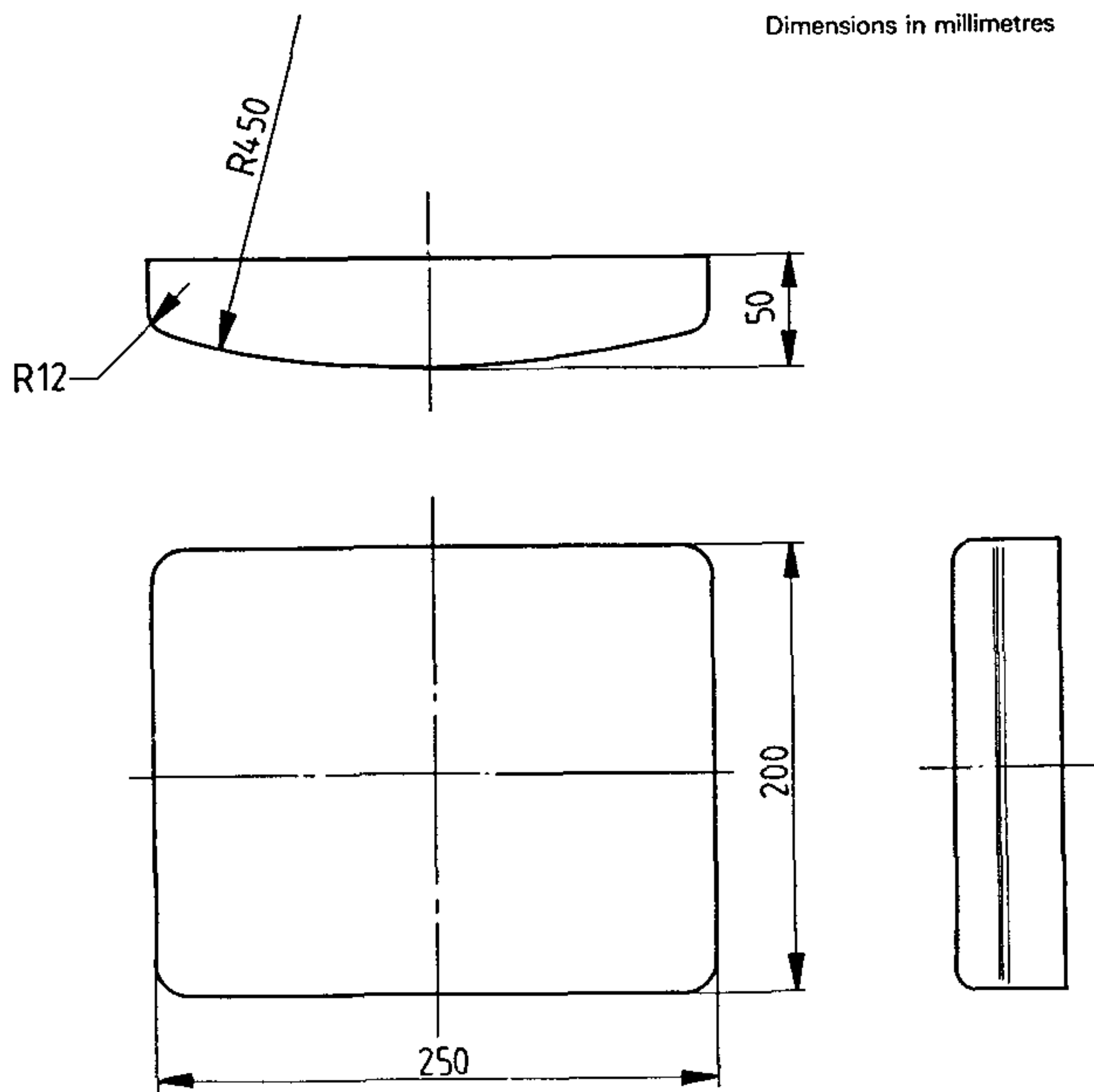
Figure 15 – Details of back loading pad
