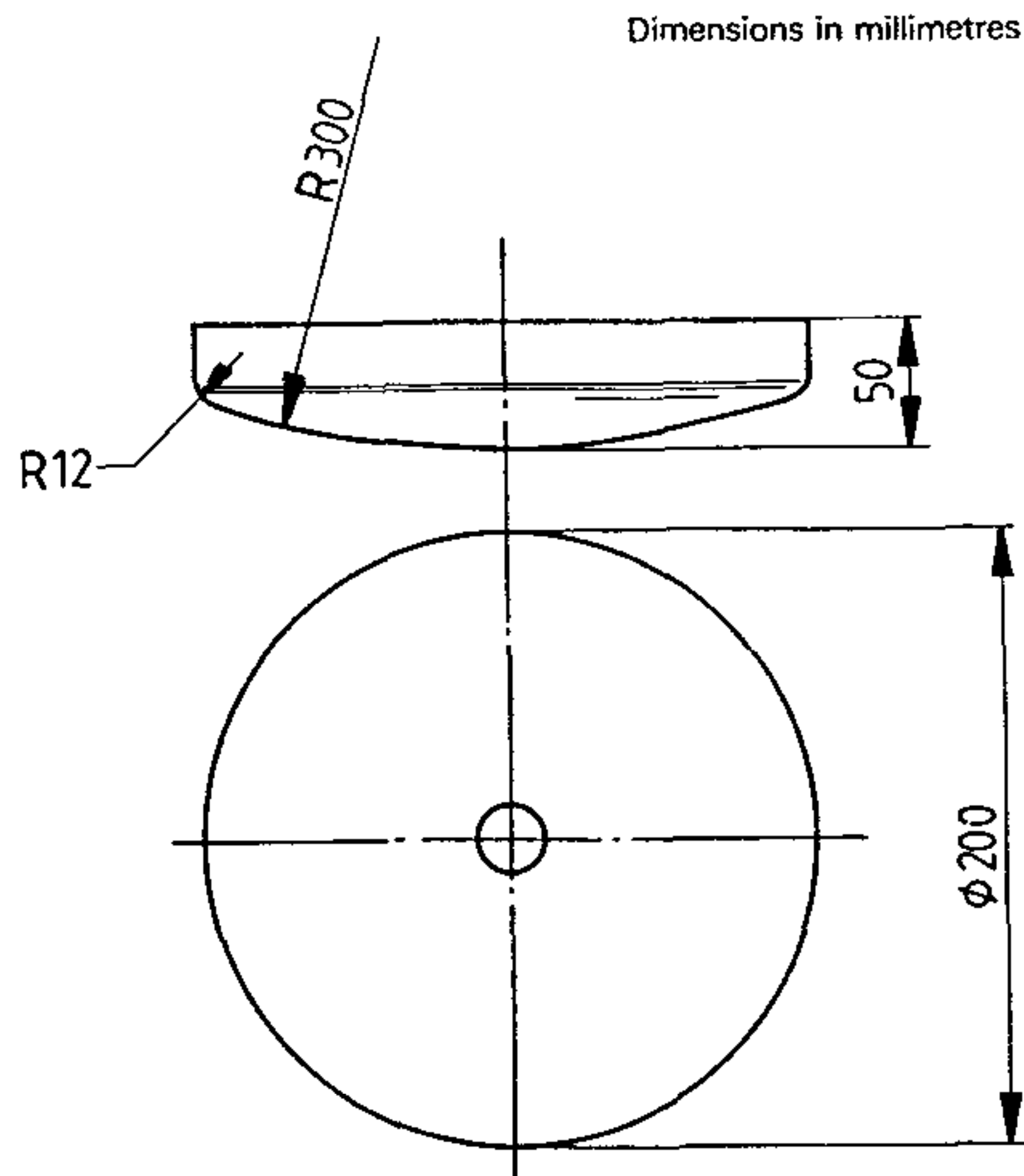
Figure 14 – Details of the smaller seat loading pad
