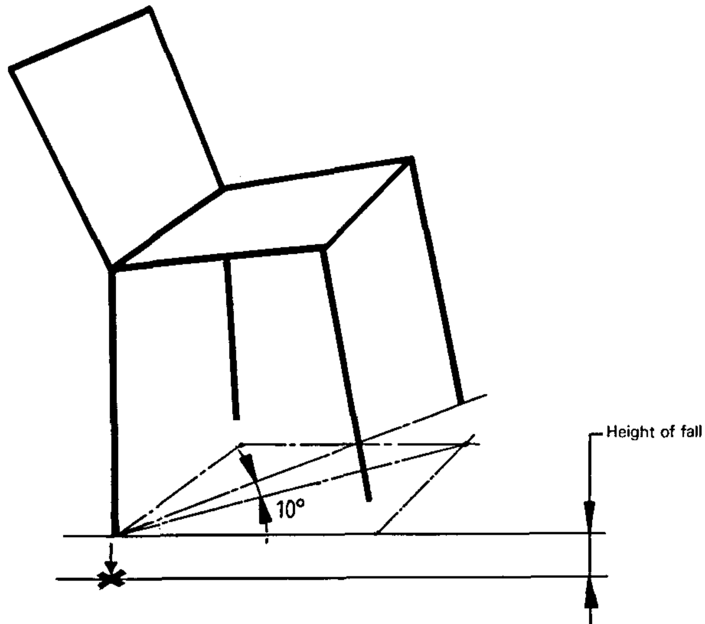
Figure 12 — Drop test
