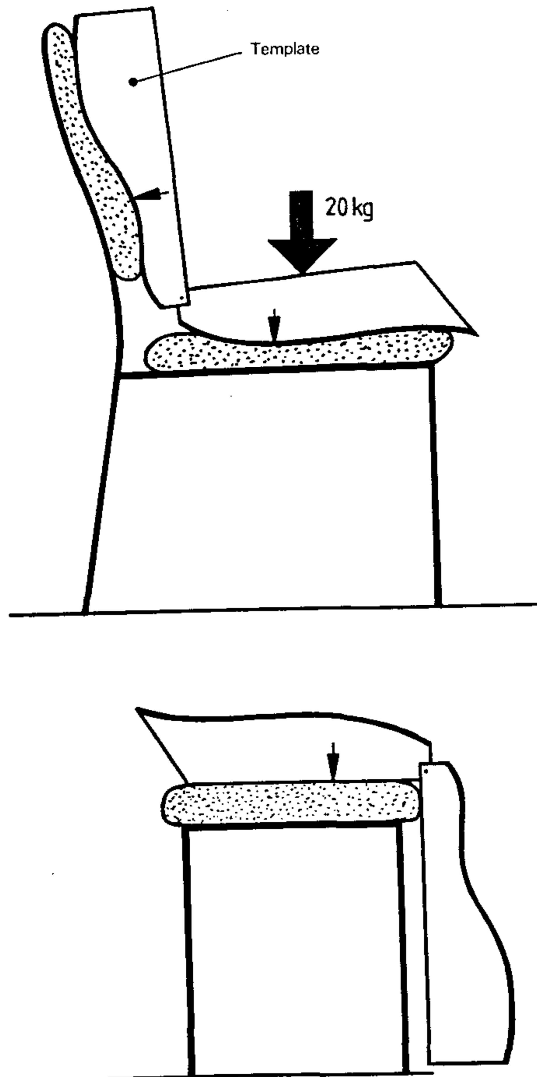
Figure 20 — Position of chair loading position template on chairs and stools
