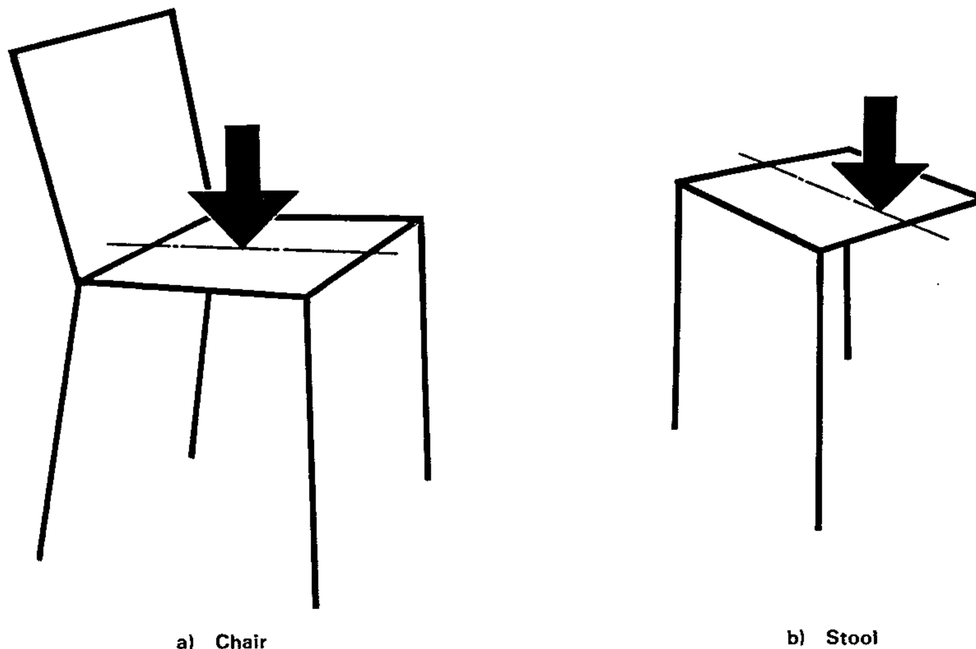
Figure 1 — Seat static load test
