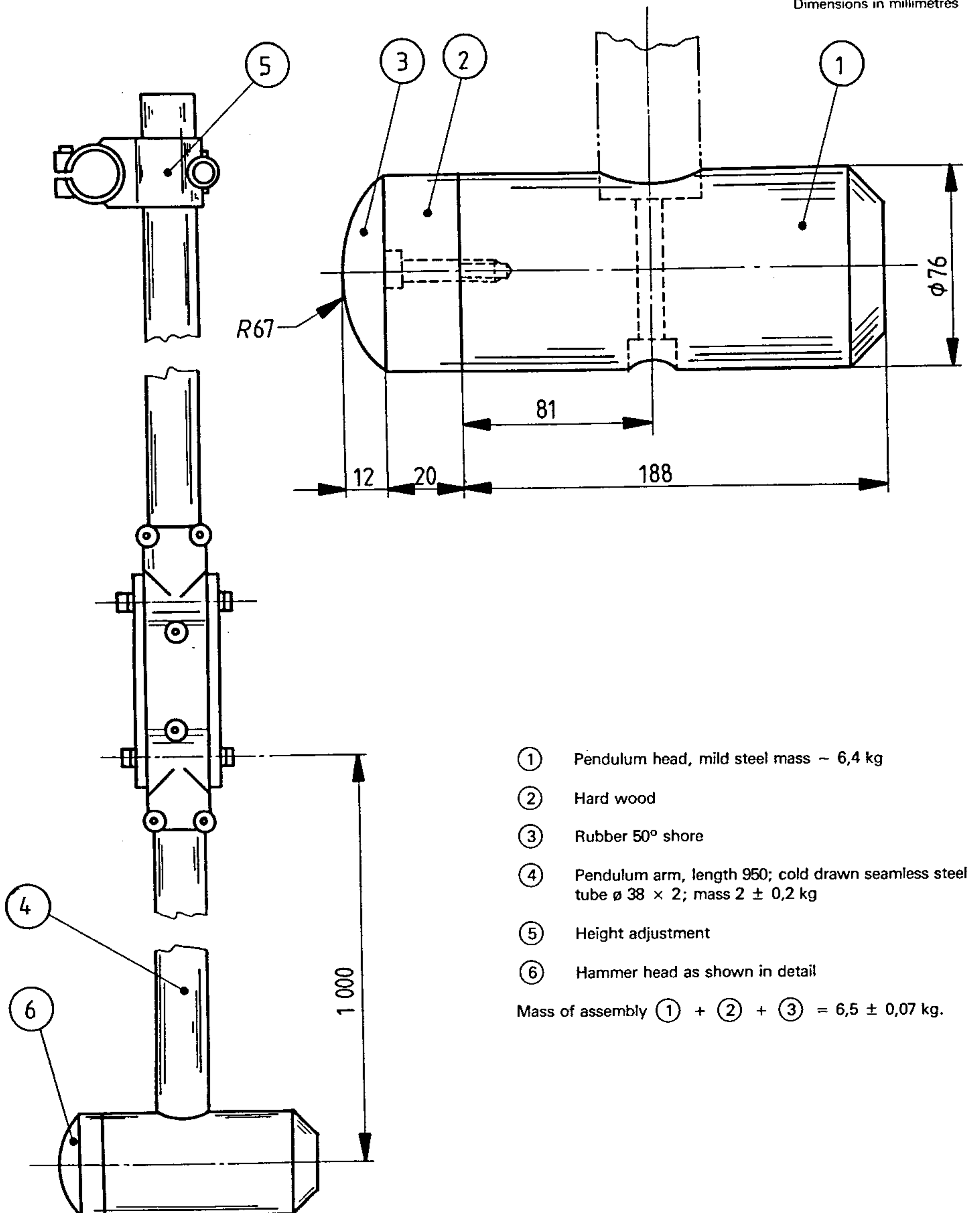
Figure 17 — Details of pendulum impact hammer
