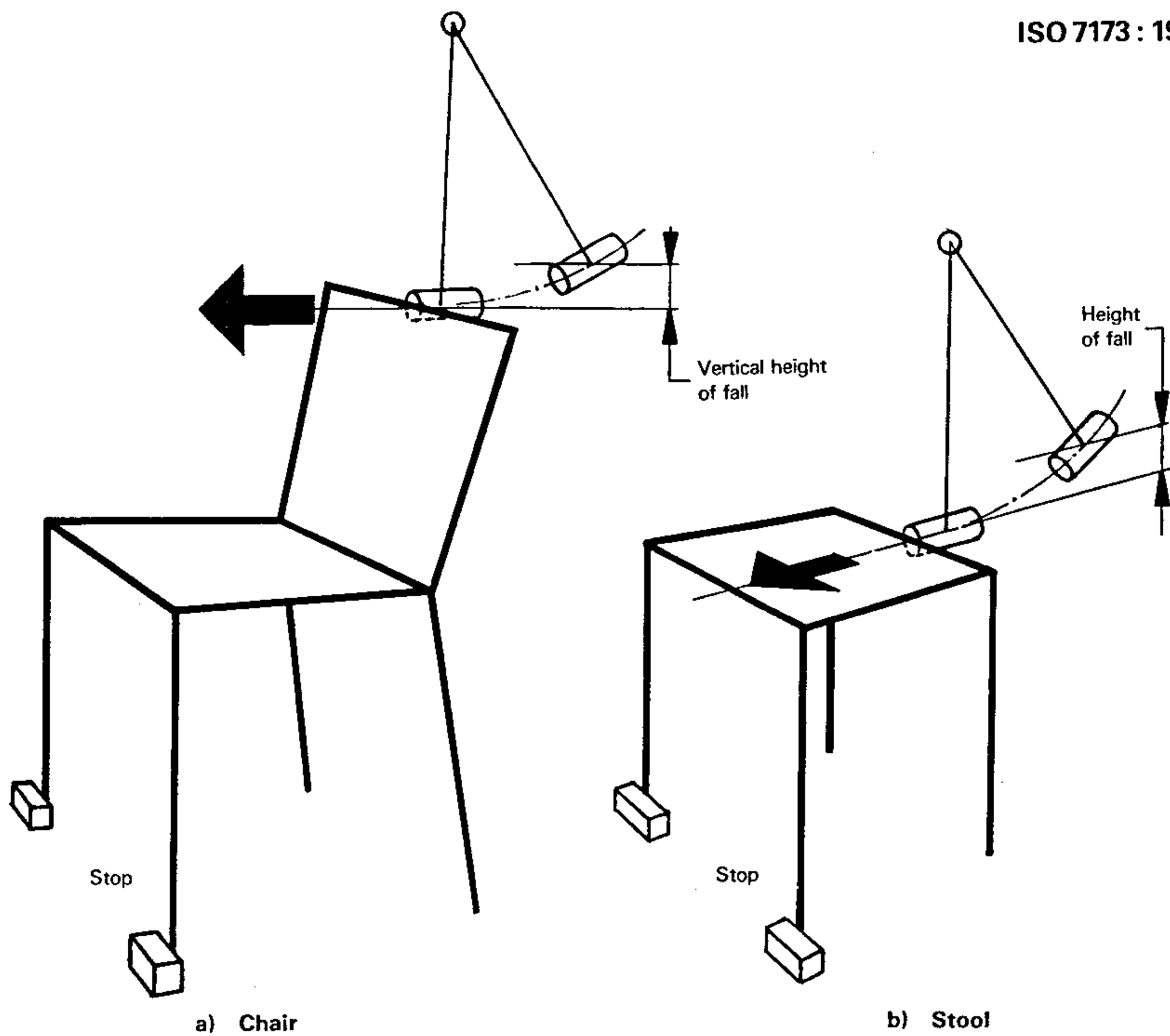
Figure 10 – Back impact test
