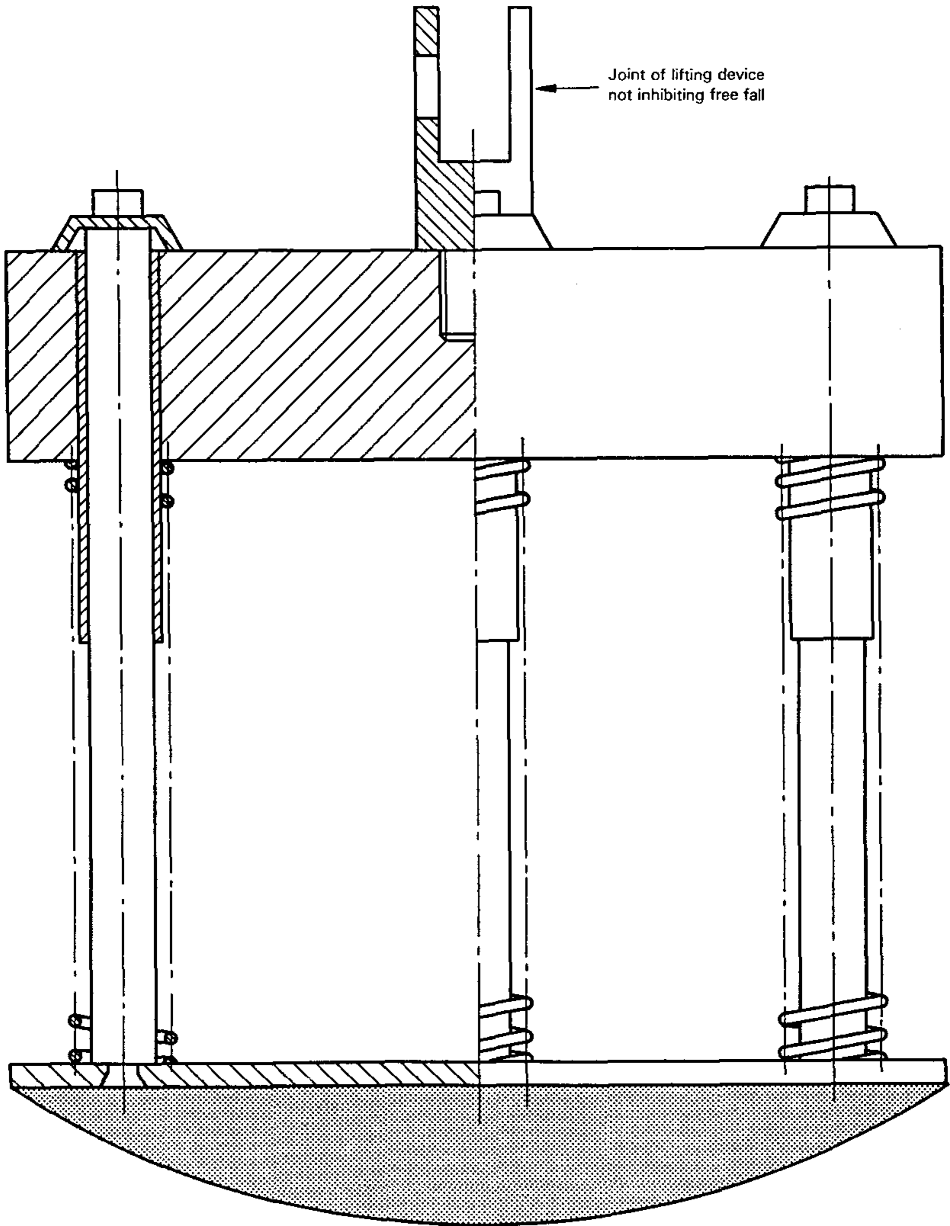
Figure 16 — Details of seat impacter
