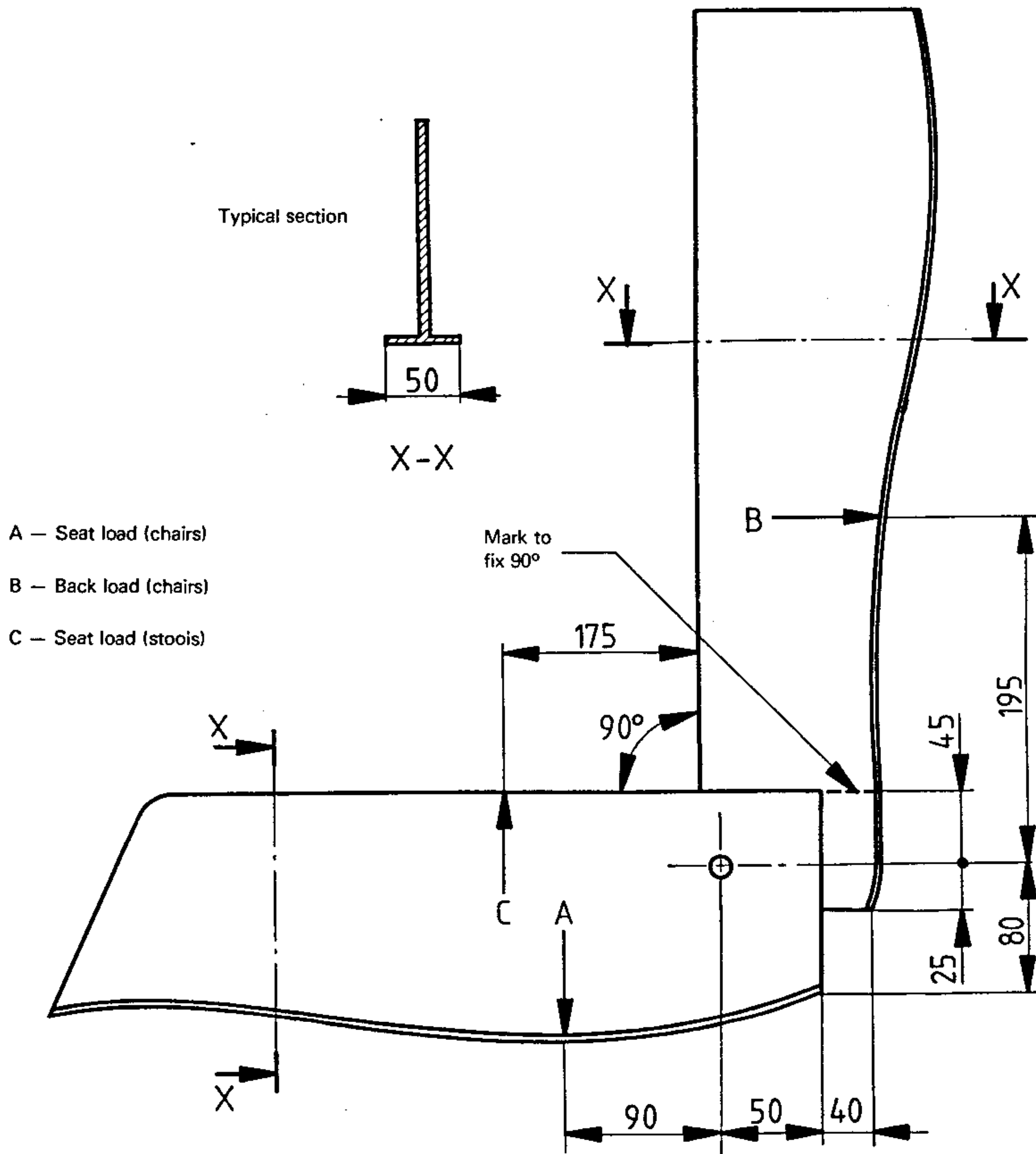
Figure 18 — Chair loading position template
