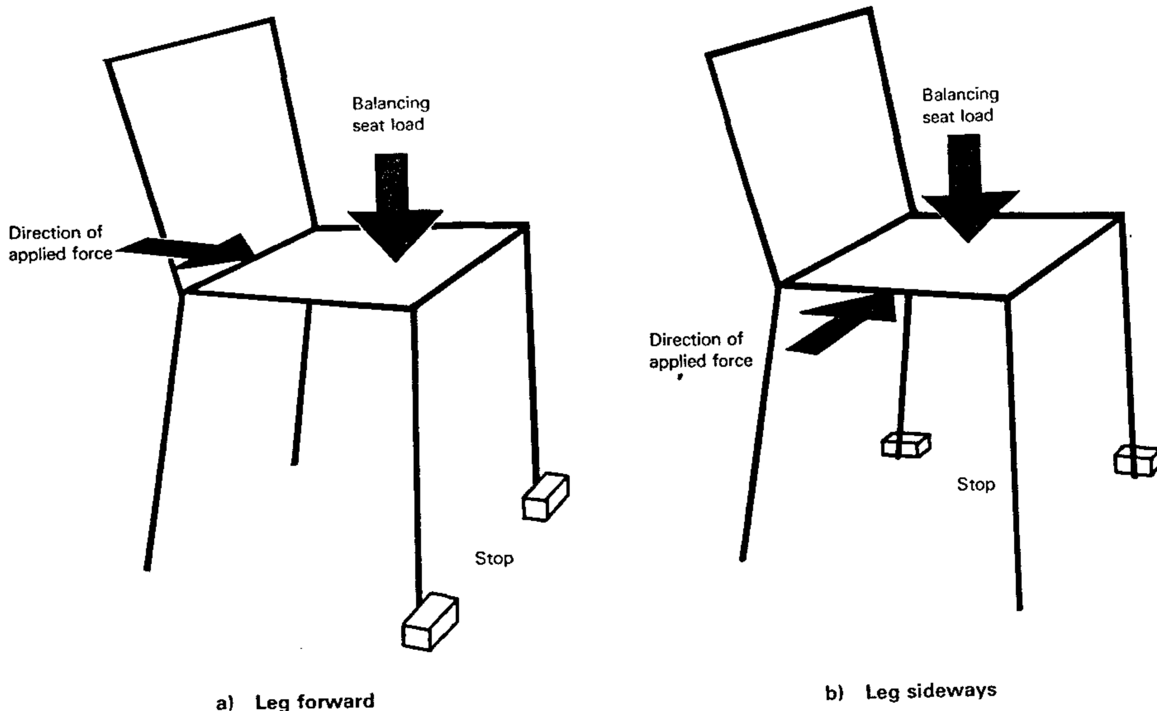
Figure 7 — Leg static load test
