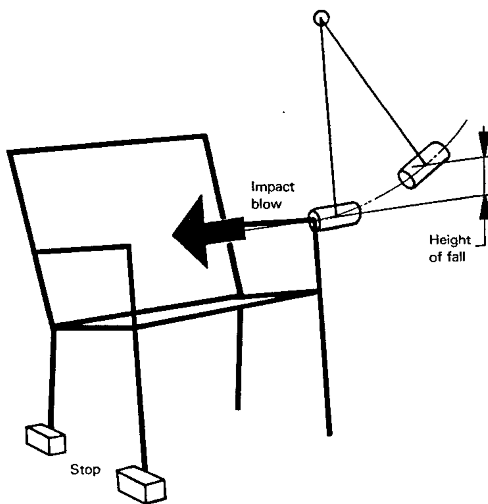
Figure 11 – Arm impact test
