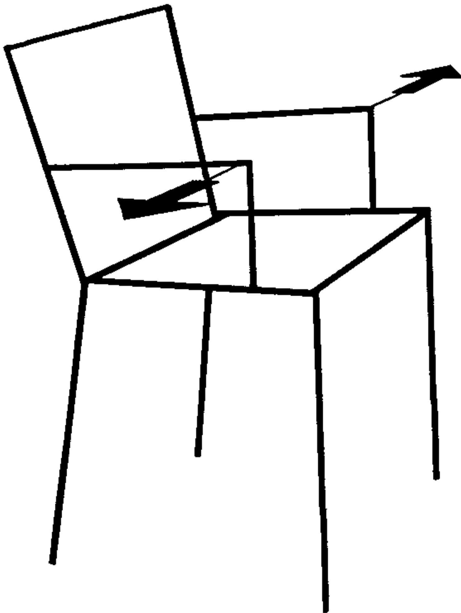
Figure 3 — Arm and wing sideways static load test
