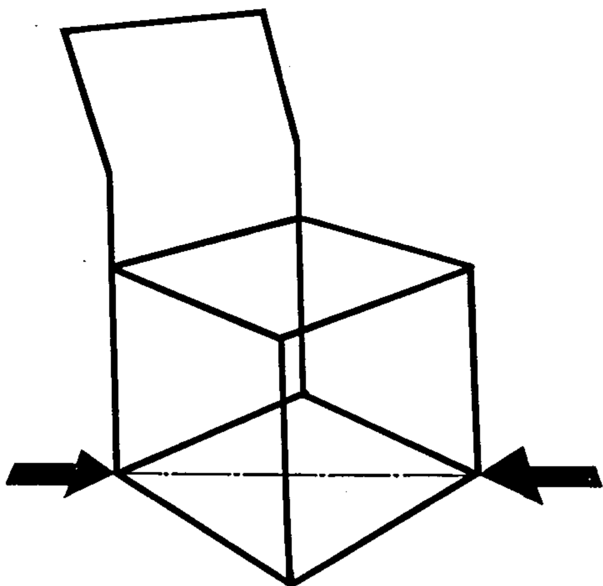
Figure 8 — Diagonal base load test — Directions of forces
