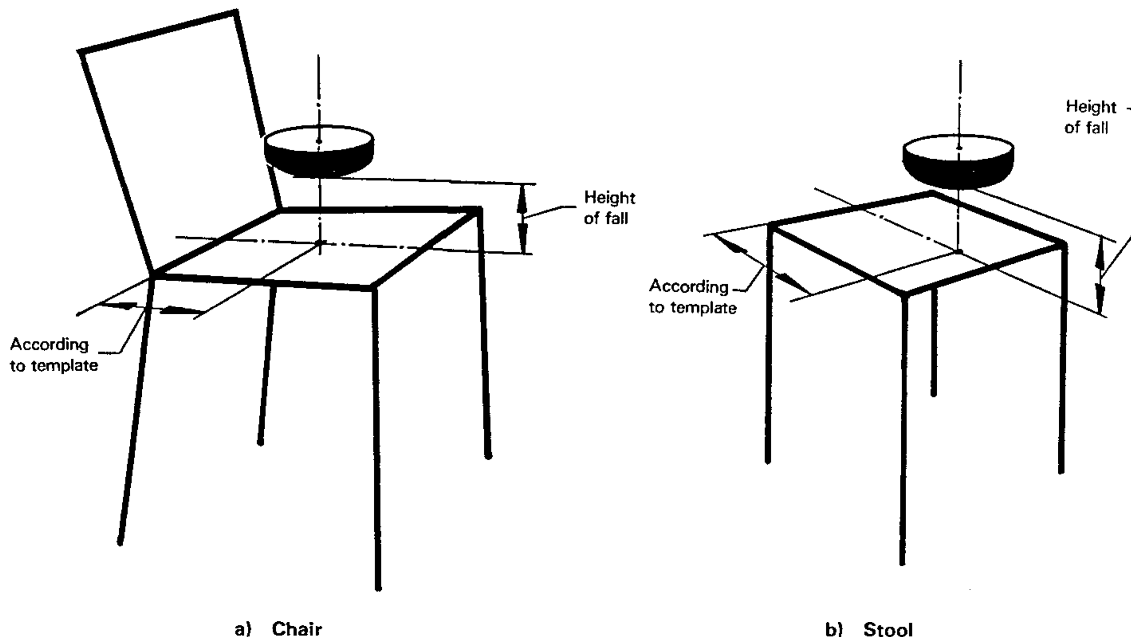
Figure 9 — Seat impact test
