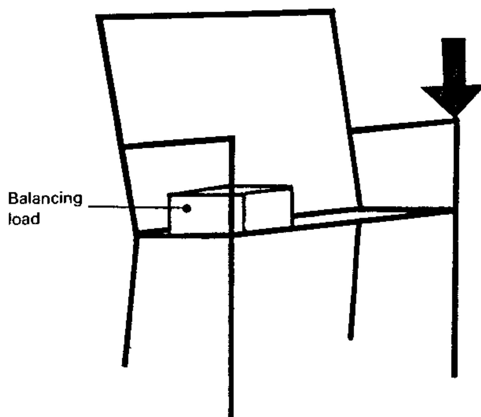
Figure 4 — Arm downwards static load test
