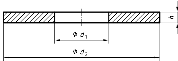
Figure 1 — Dimensions
