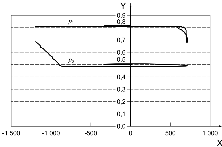
Figure D.3 — Pressure response during discharge
