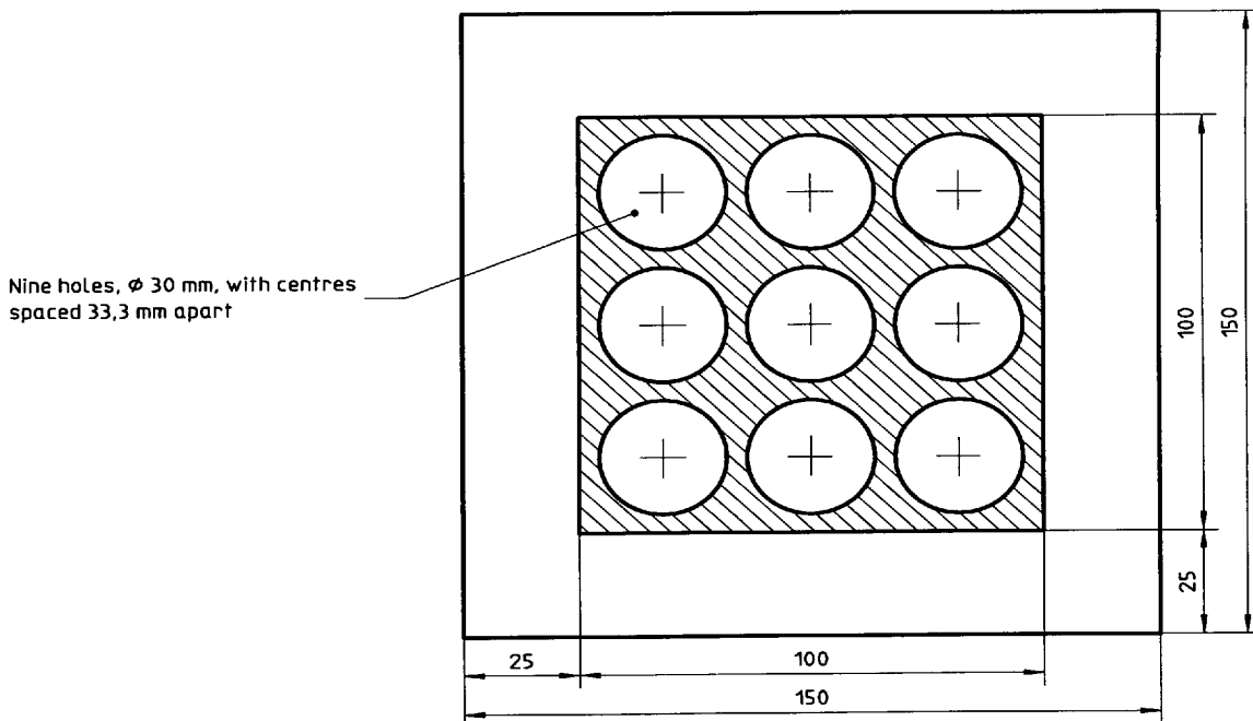
Figure 1 — Locations from which standard test pieces are to be cut when testing standard test slabs or commercial flat sheets
