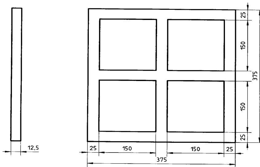
Figure 2 — Four-cavity frame for standard test slabs of cellular rubbers
