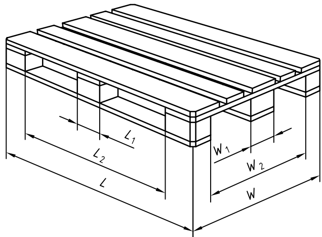
f) Entries: four-way pallet
