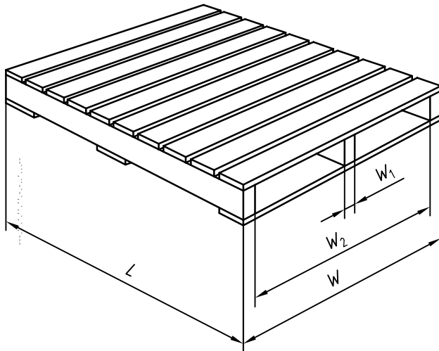
c) Entries: non-reversible two-way pallet
