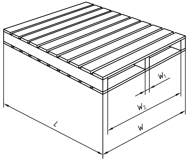
b) Entries: reversible two-way pallet
