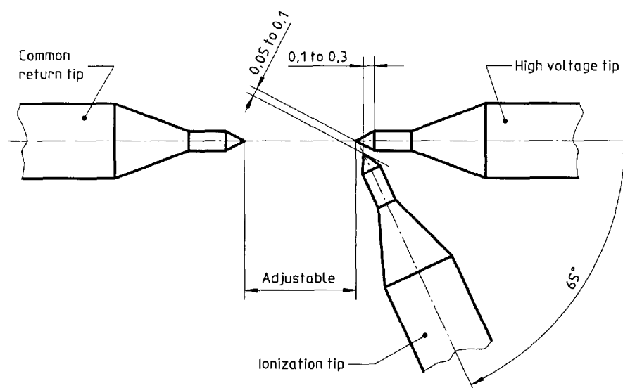
Figure 5 — Setting of pointed spark gap
