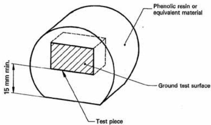
Figure 2 — Embedded test piece with one test surface
