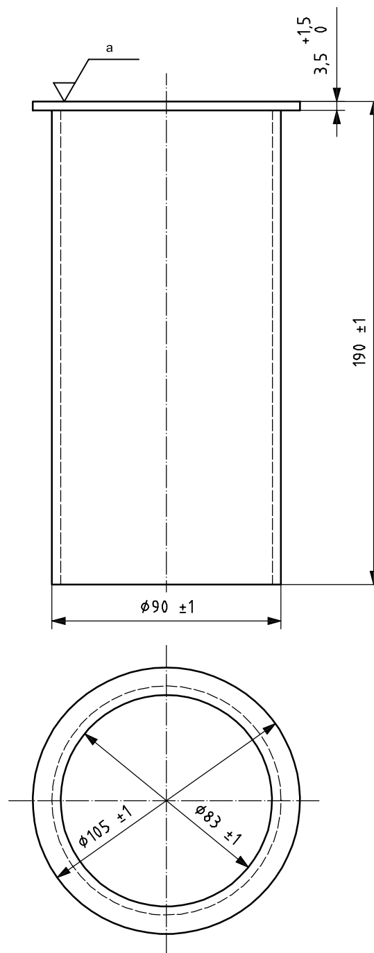
Figure 1 — Glass beaker
