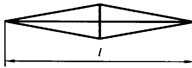
Figure 1 — Knoop indenter
