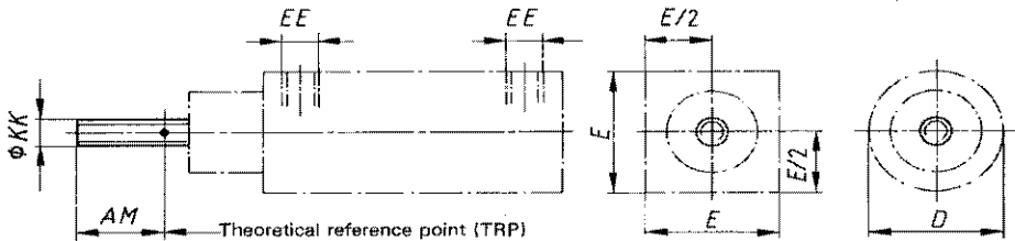
Figure 1 — Basic dimensions
