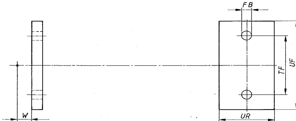
Figure 2 — Head rectangular flange (two hole) mounting (MF8)
