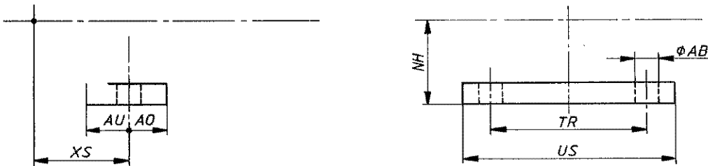
Figure 5 – Head angle mounting (MS3)
