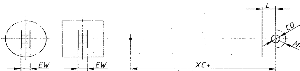
Figure 3 — Cap fixed eye mounting (MP3)
