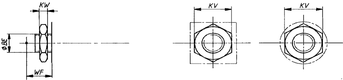
Figure 4 – Head threaded mounting (MR3)
