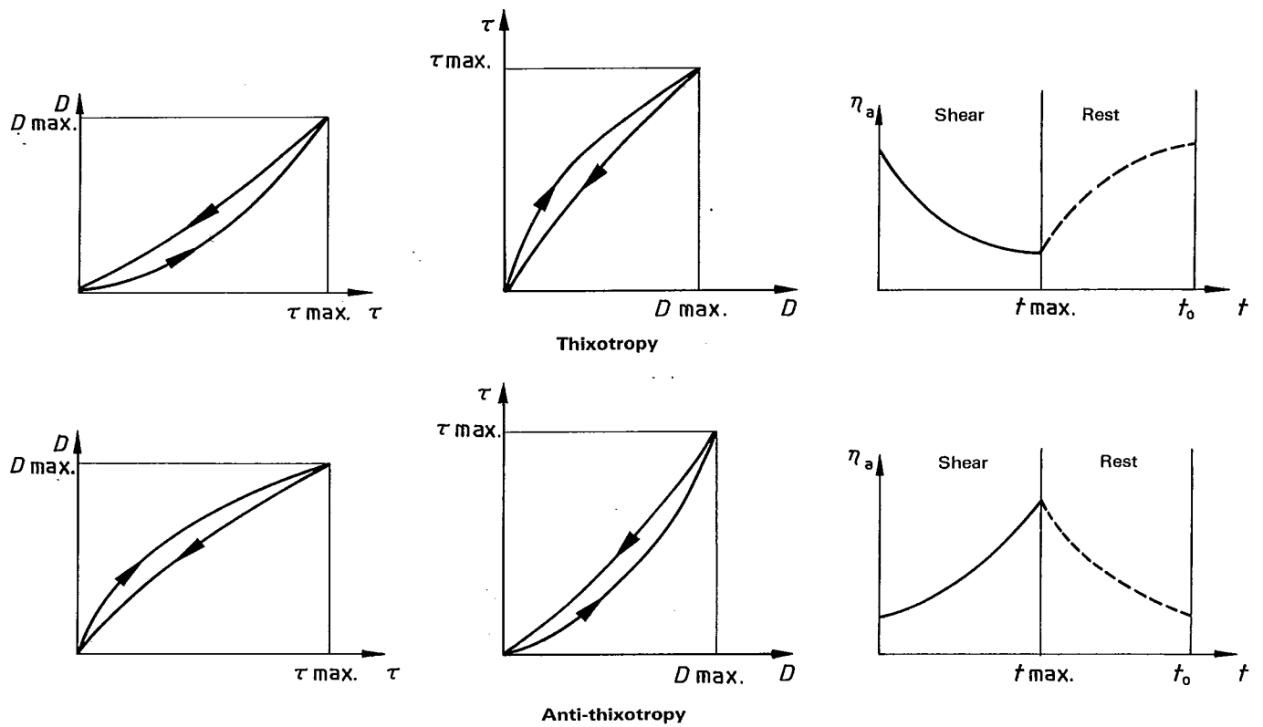
Figure 2 — Representation of a hysteresis curve for a product which is strongly affected in its rheological behaviour by the length of time for which the shear is applied.
