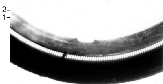
Figure 9 — Nick
