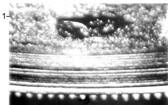
Figure 3 — Inclusion: flash
