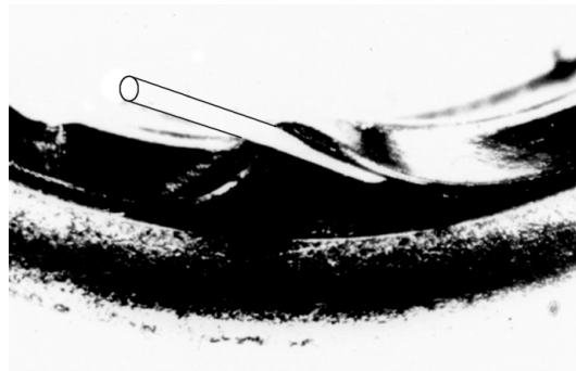
Figure 26 — Incomplete bond
