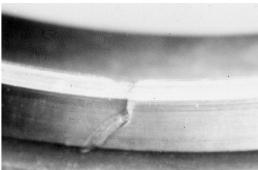
Figure 29 — Non-fill
