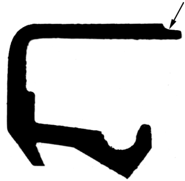
Figure 25 — Incorrect lead-in chamfer on seal outside diameter
