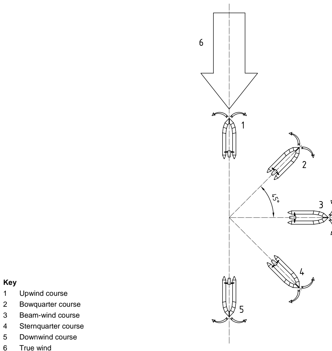
Figure 3 — In-water performance test
