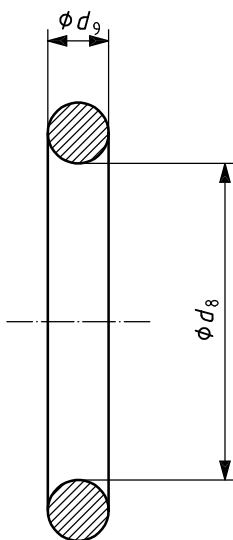
Figure 3 — O-ring
