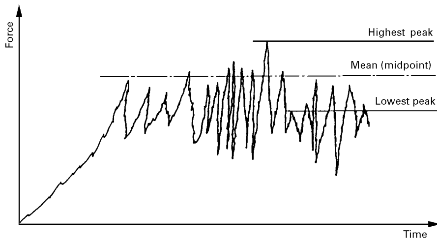
Figure 4 – Analysis of a trace with a large number of peaks (too close for counting)
